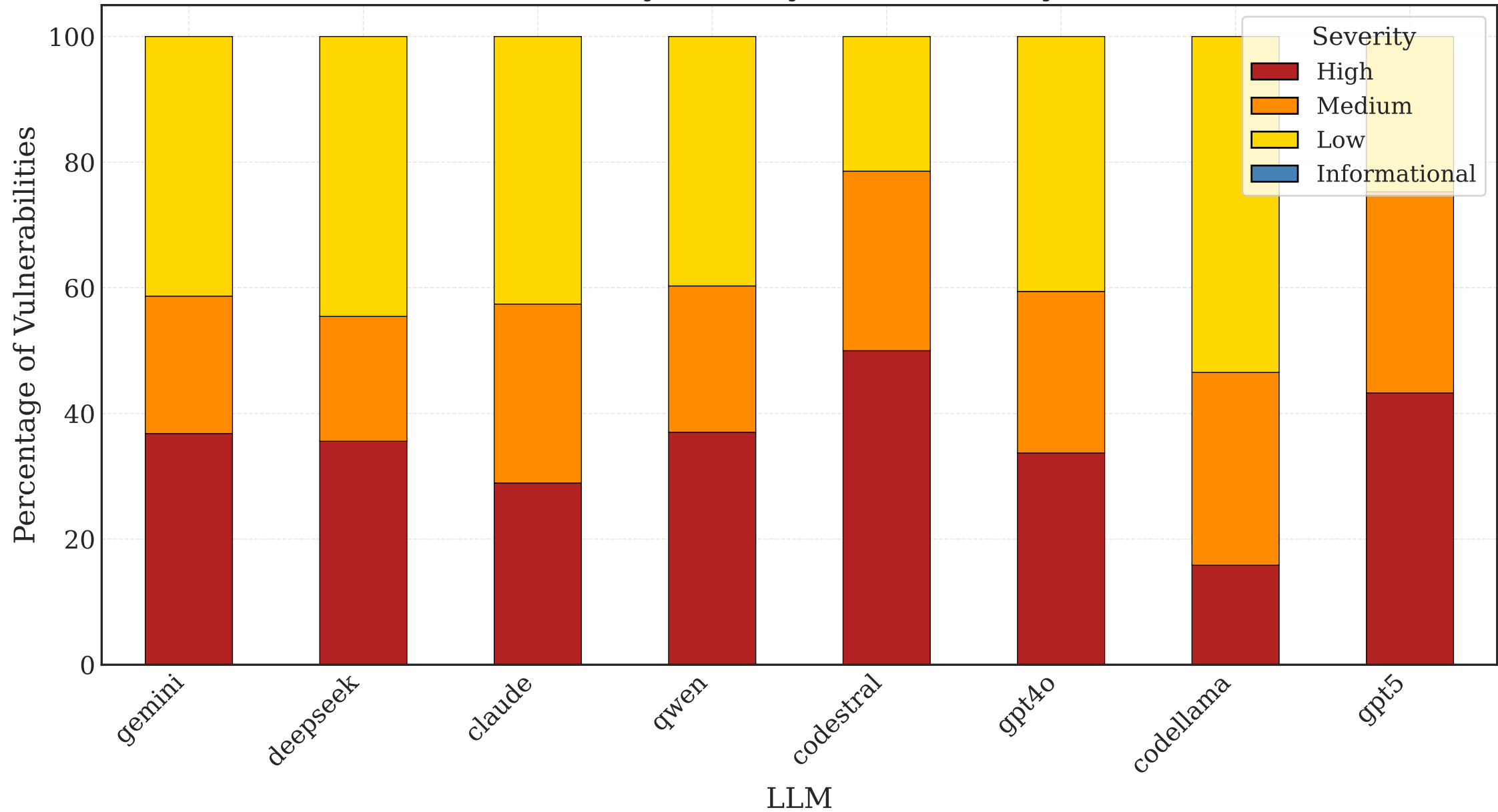
Vulnerability Severity Distribution by LLM
