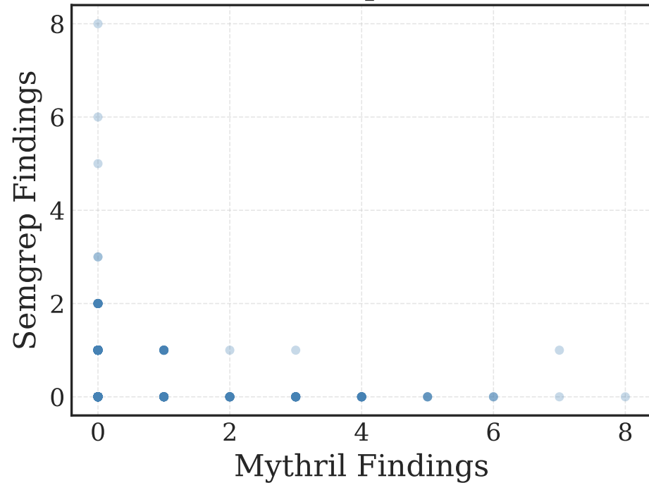
Mythril vs Semgrep (rho=0.047, p=2.27e-02)
