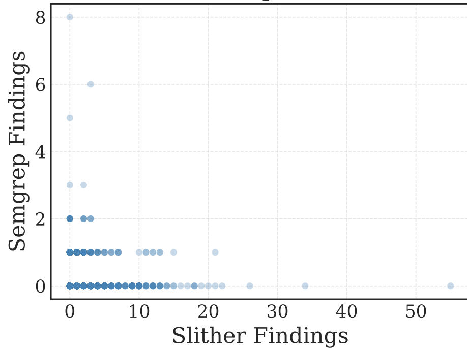
Slither vs Semgrep (rho=0.129, p=2.25e-10)
