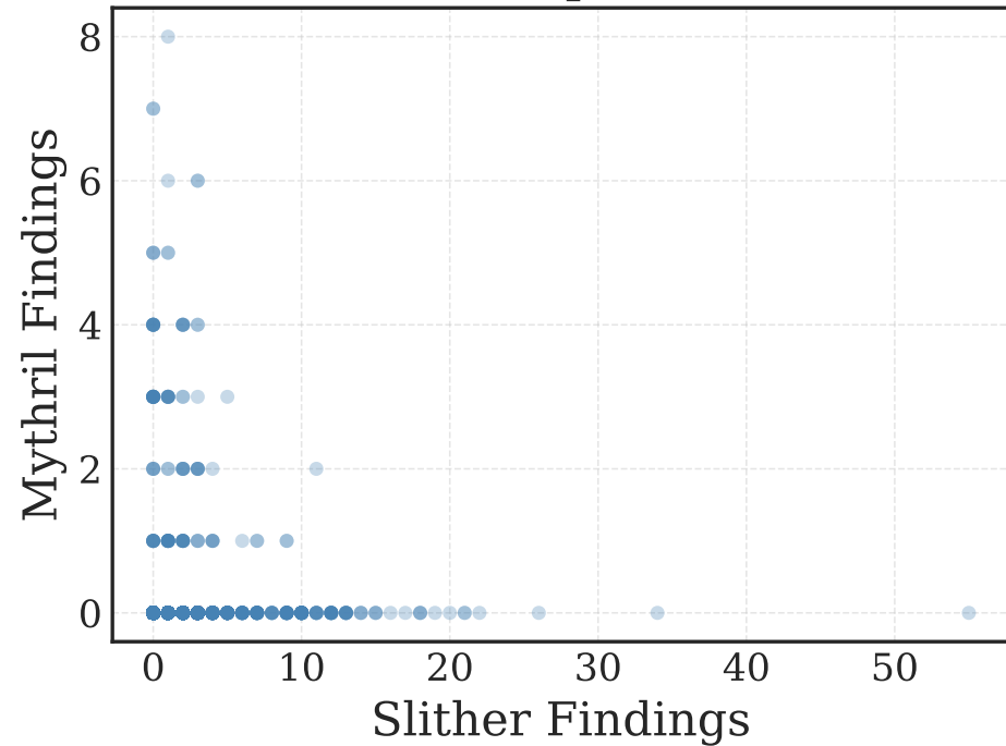
Slither vs Mythril (rho=0.134, p=4.20e-11)
