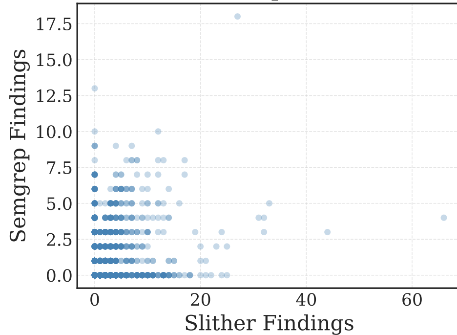
Slither vs Semgrep (rho=0.307, p=1.51e-53)
