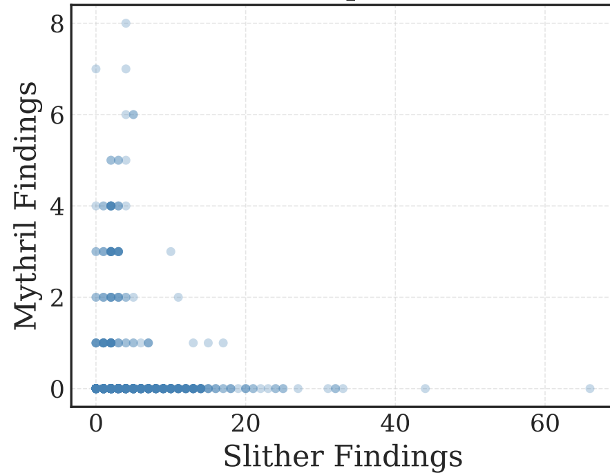
Slither vs Mythril (rho=0.185, p=5.17e-20)
