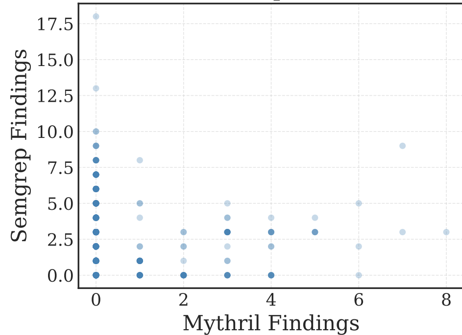
Mythril vs Semgrep (rho=0.141, p=3.83e-12)
