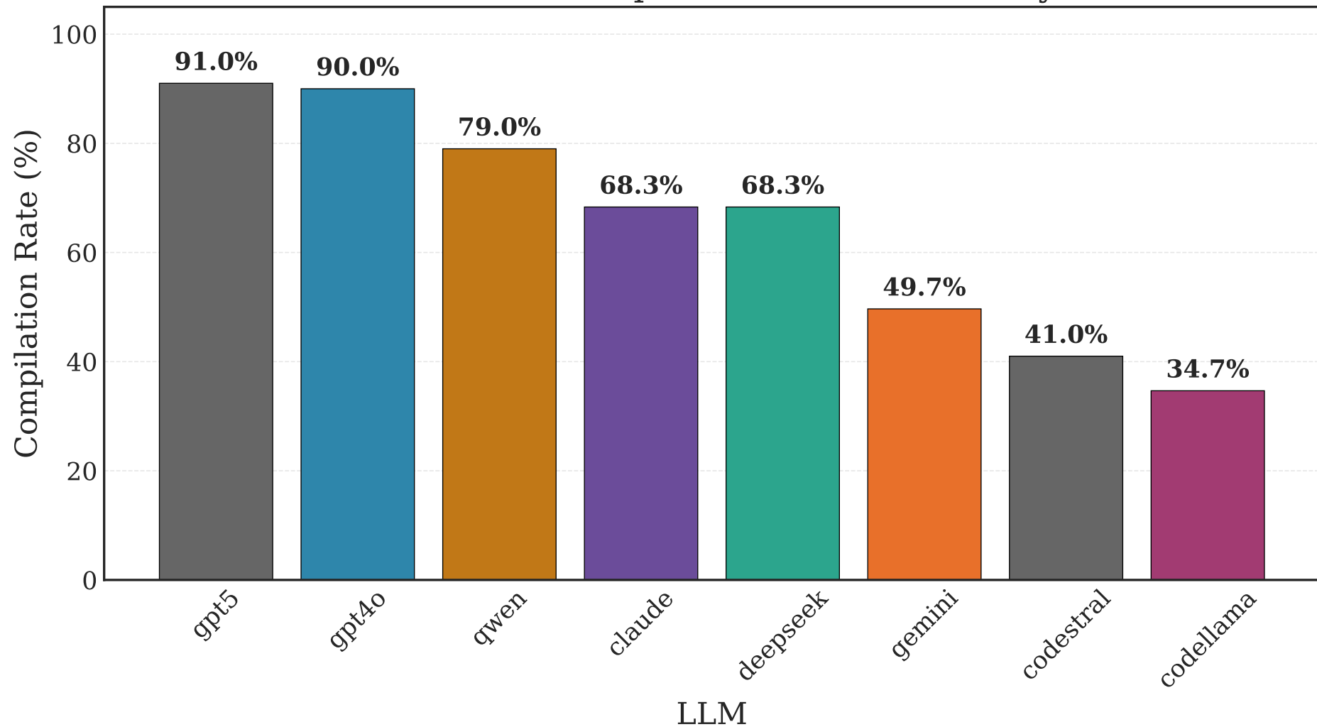
Smart Contract Compilation Success Rate by LLM
