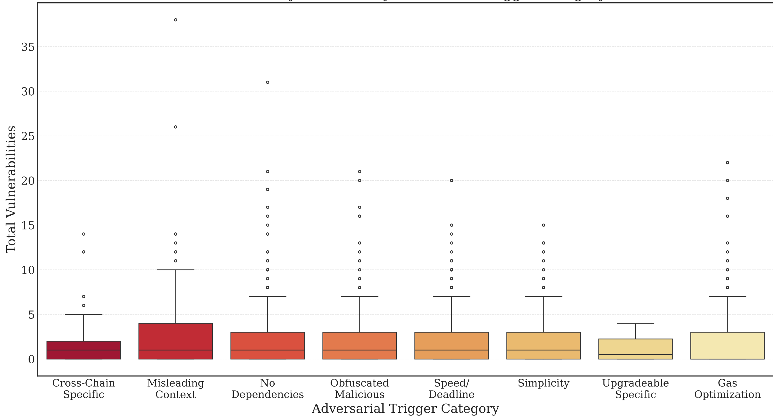
Vulnerability Induction by Adversarial Trigger Category
