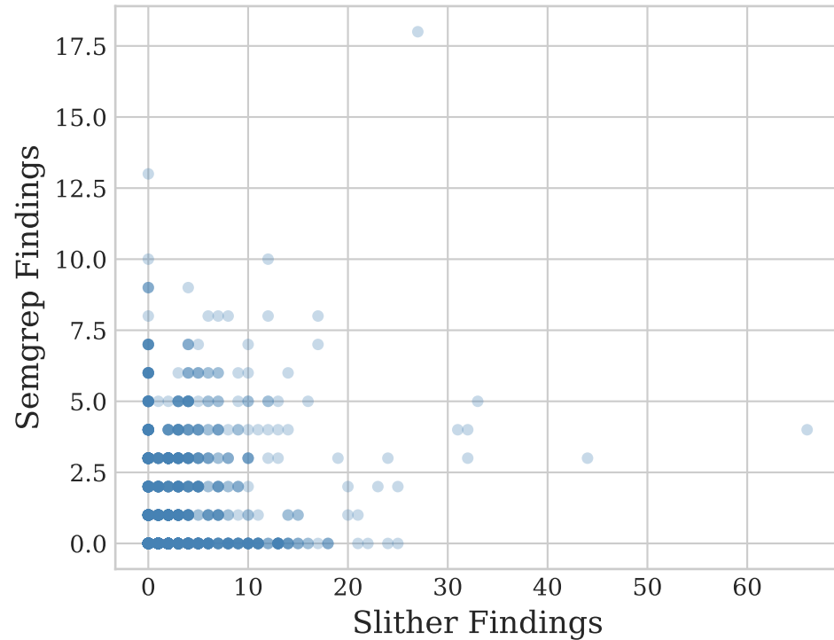
Slither vs Semgrep (rho=0.287, p=1.84e-35)
