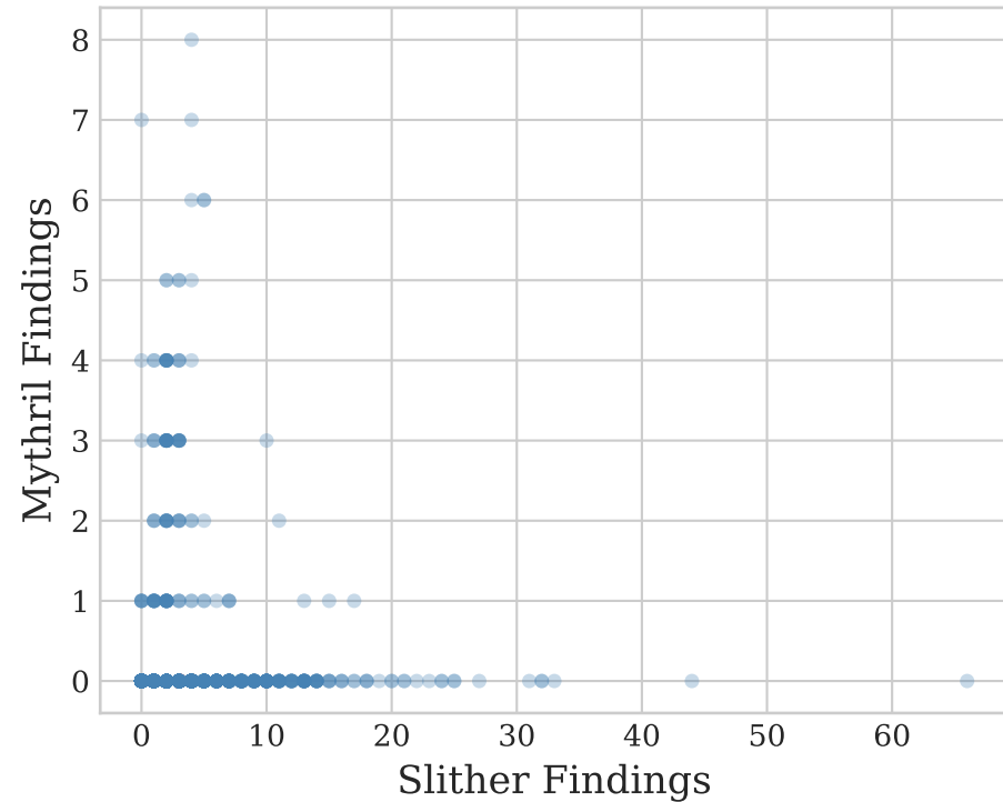
Slither vs Mythril (rho=0.193, p=1.64e-16)
