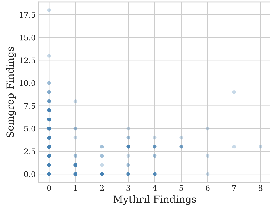
Mythril vs Semgrep (rho=0.142, p=1.61e-09)
