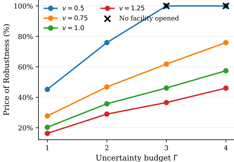
(c) Average-Case Robustification Value
