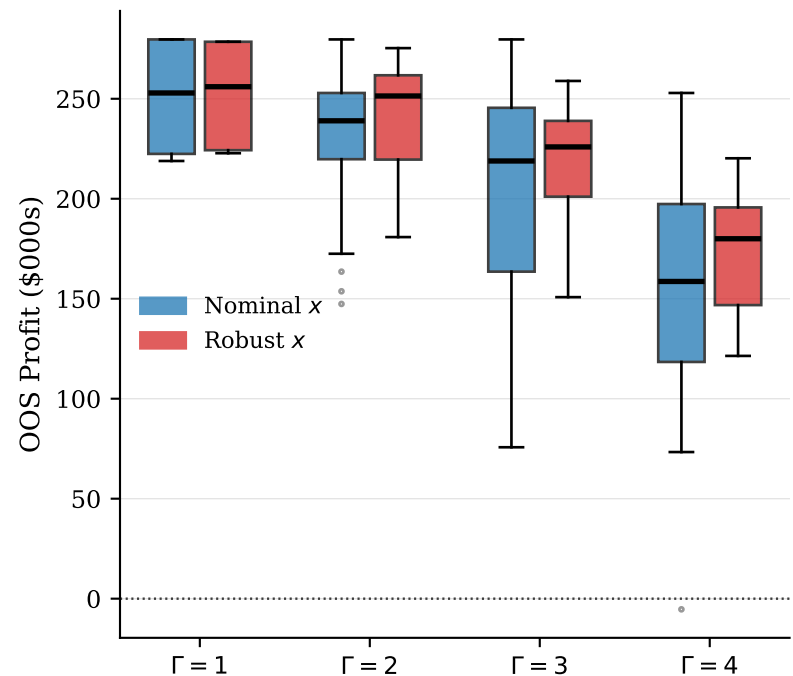
(c) OOS Profit Distribution: Adaptive Pricing
