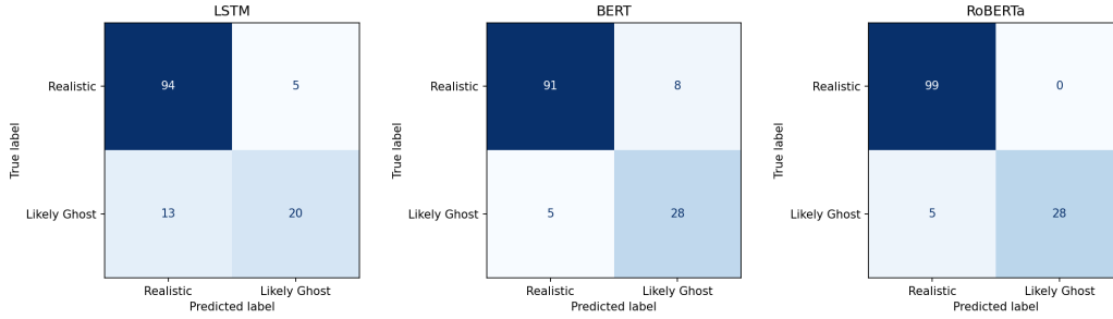
Figure 3.2: Confusion matrices for the three ghost-job classification models.
