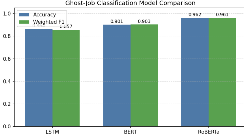
Figure 3.1: RoBERTa achieves the highest accuracy and weighted F1 on ghost-job risk classification.
