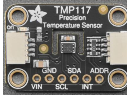
Ek 1 TMP 117 Temprature Sensor
