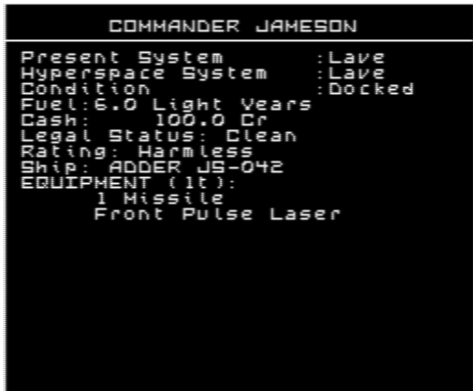
Starting Commander
