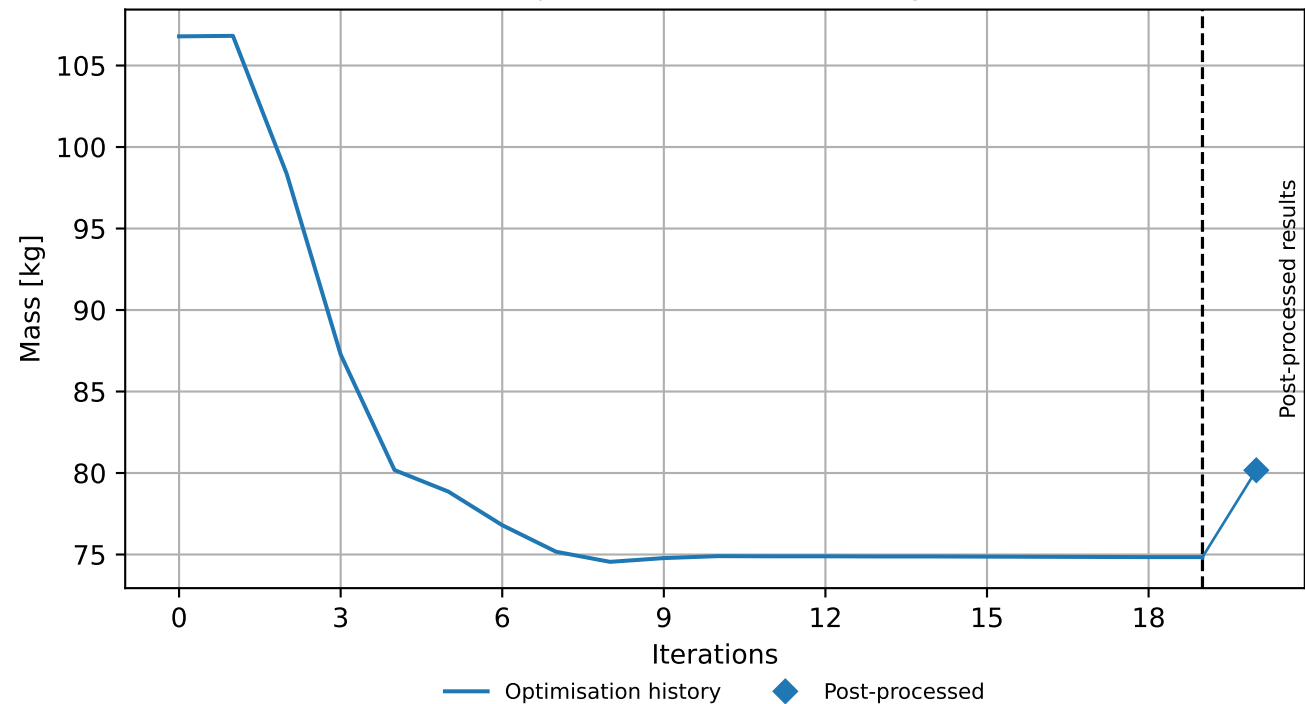
SLP Objective function convergence
