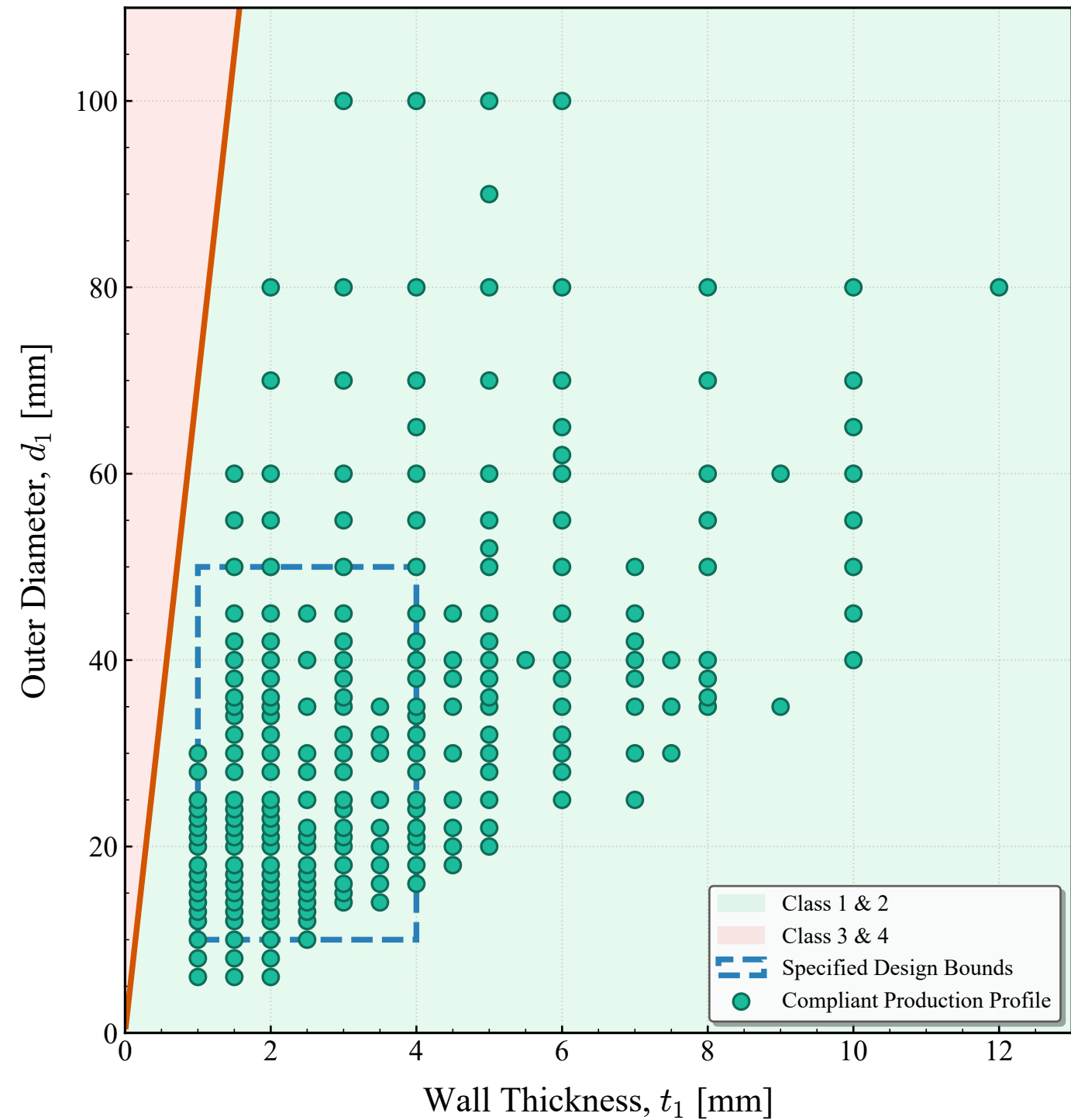
S235 Braces (Production Profiles & Initial Bounds)
