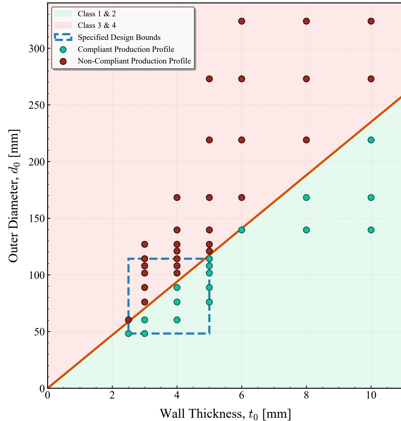
Strenx 700 Columns (Production Profiles & Initial Bounds)
