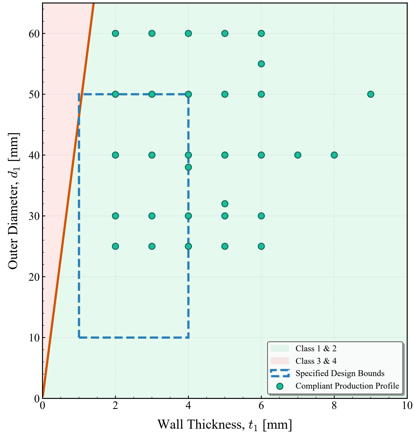
S355 Braces (Production Profiles & Initial Bounds)
