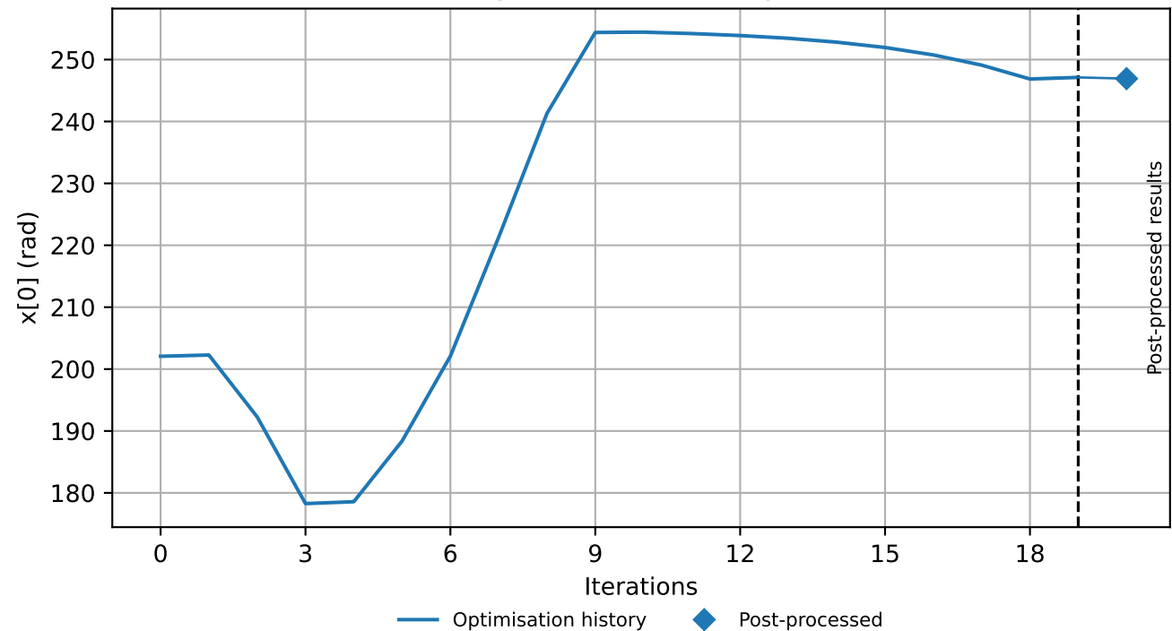
SLP Design variable convergence: rad
