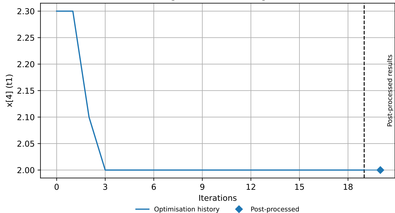
SLP Design variable convergence: t1
