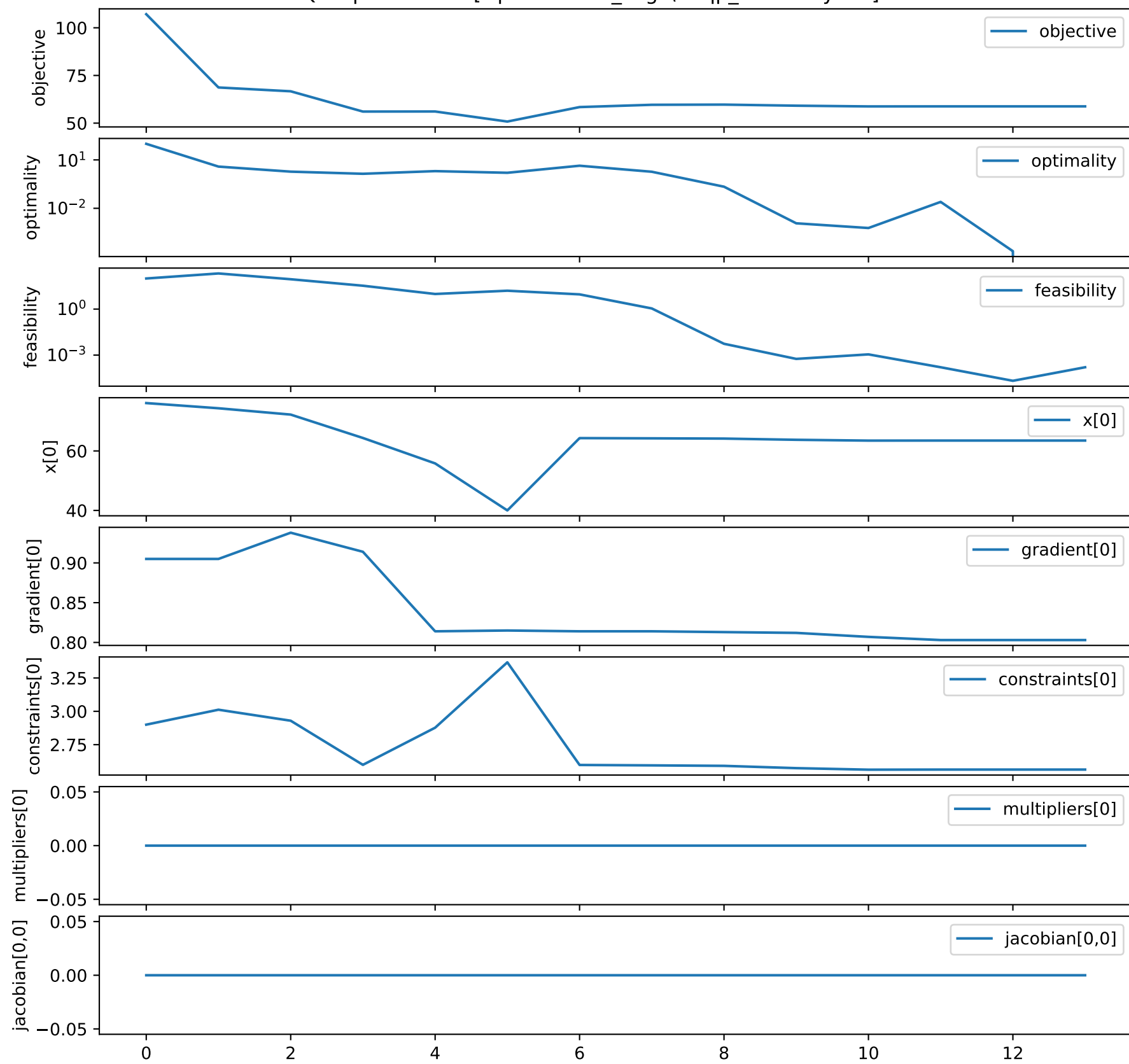
SLSQP Optimization [Optimization_Logs\slsqp_summary.out]
