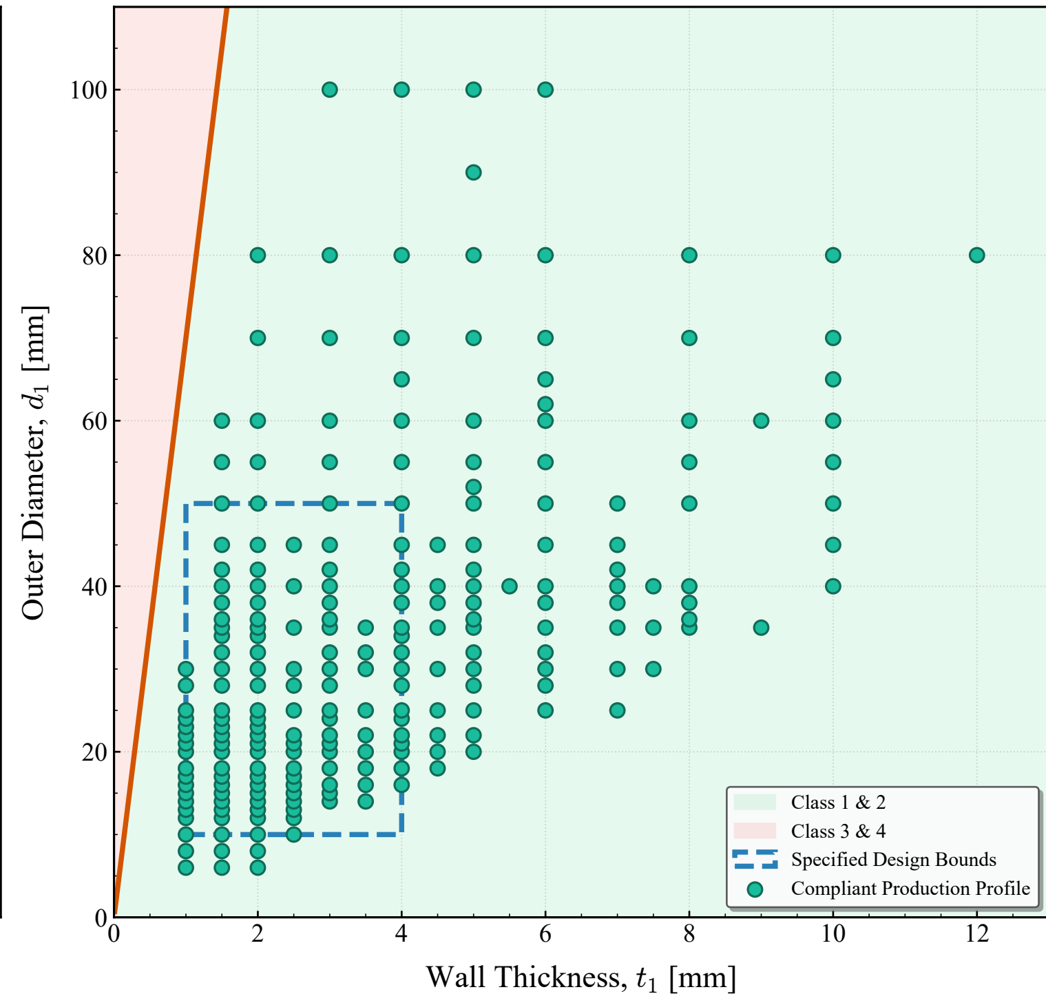
S235 Braces (Production Profiles & Initial Bounds)
