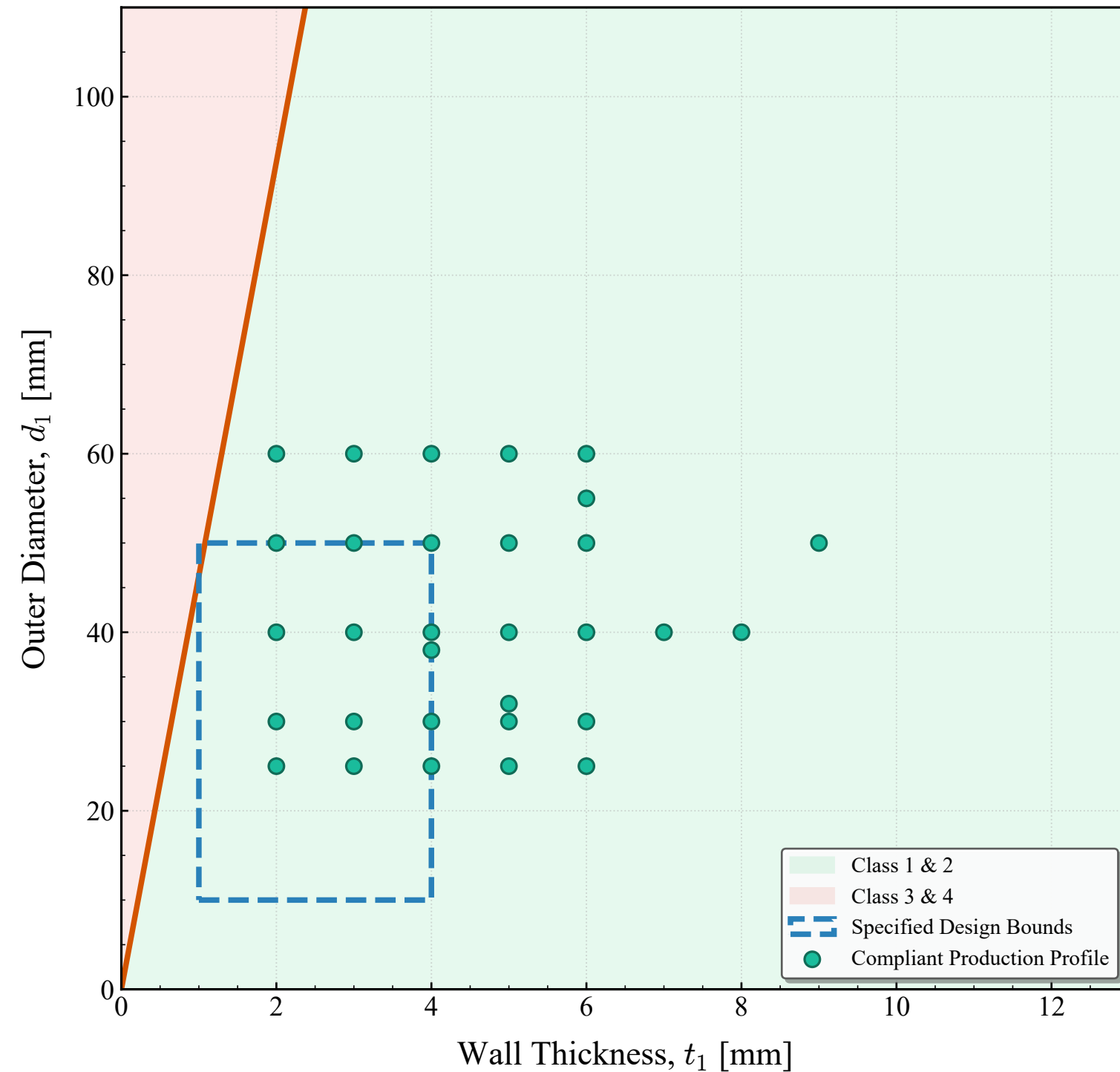
S355 Braces (Production Profiles & Initial Bounds)
