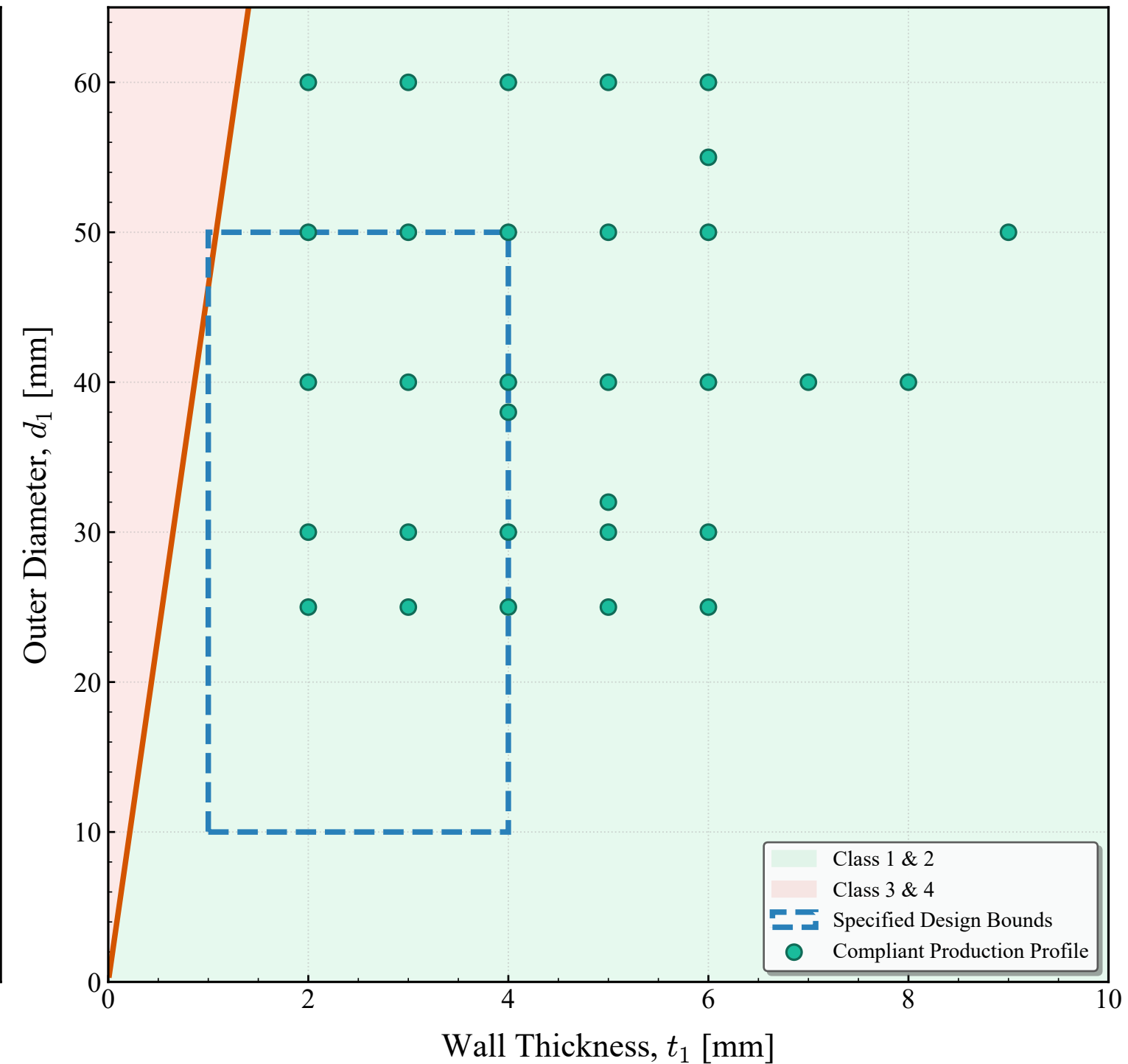
S355 Braces (Production Profiles & Initial Bounds)
