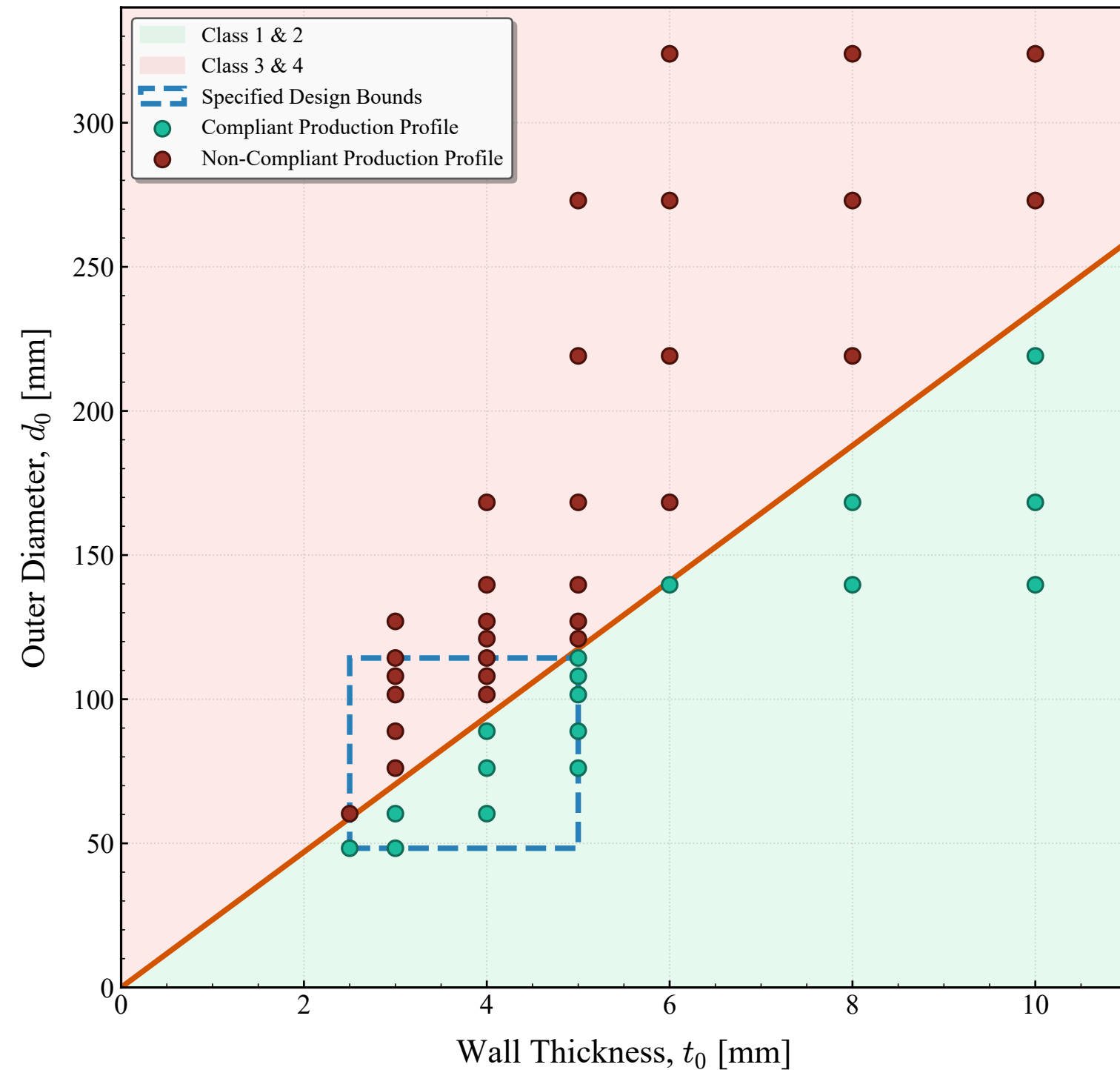
Strenx 700 Columns (Production Profiles & Initial Bounds)
