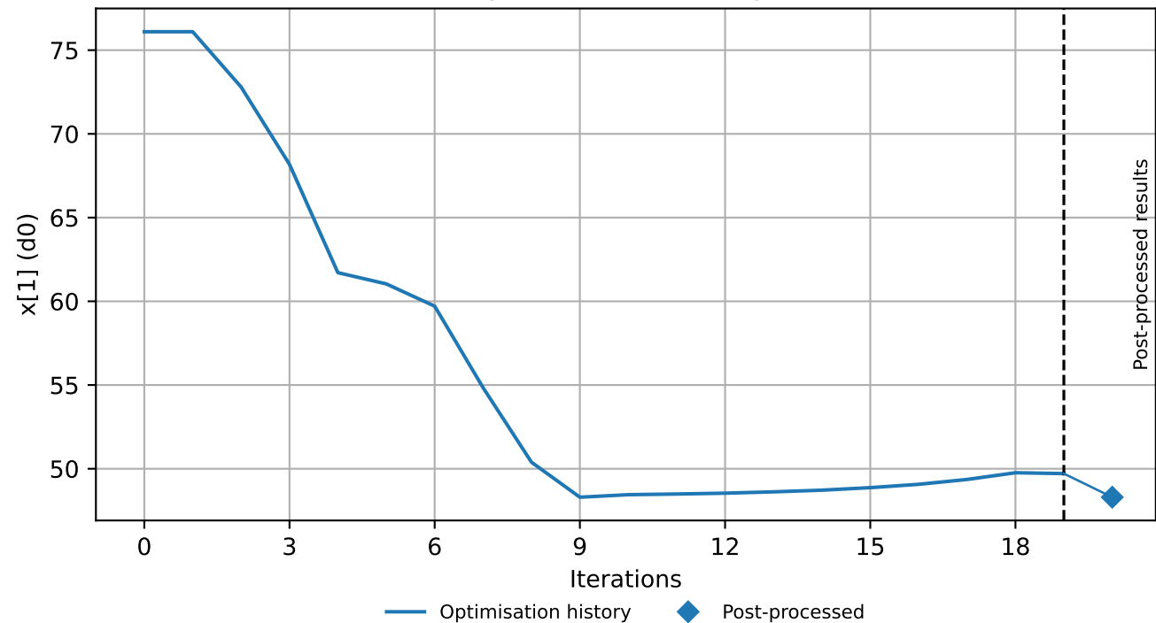
SLP Design variable convergence: d0
