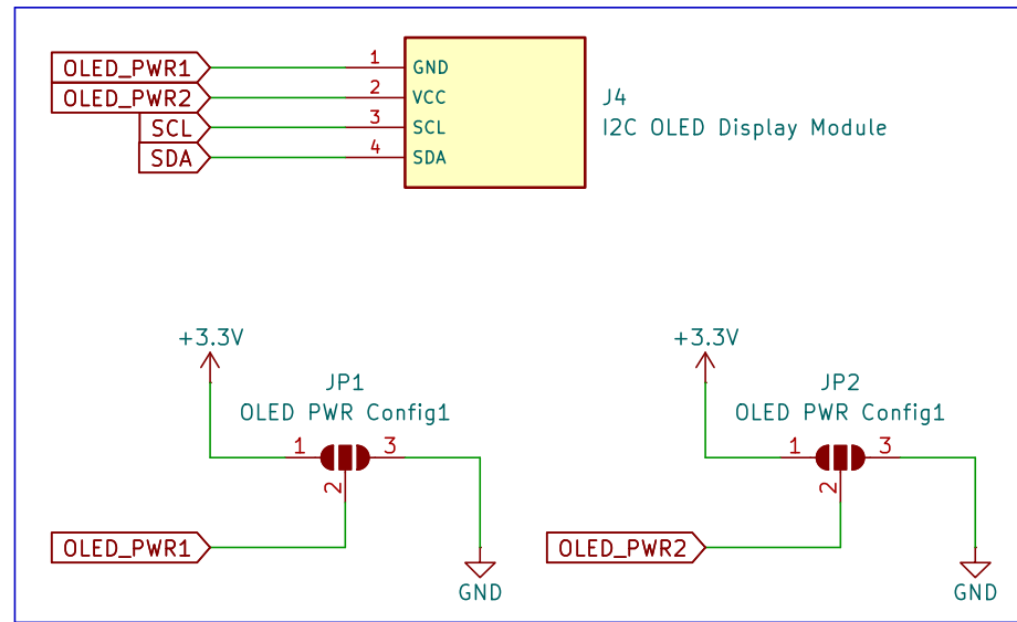
I2C OLED Display Module Connector with configurable Power Input
