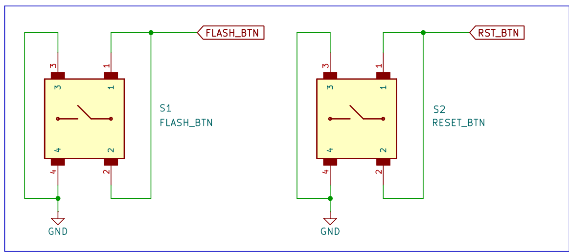
Main Board Flash and Reset Buttons
