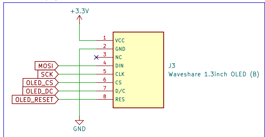
SPI OLED Display Module Connector
