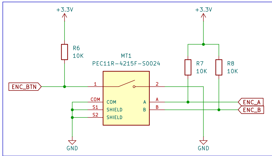
Rotary Encoder
