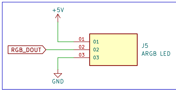
ARGB LED Connector
