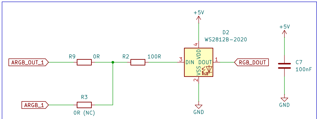
RGB Status LED
