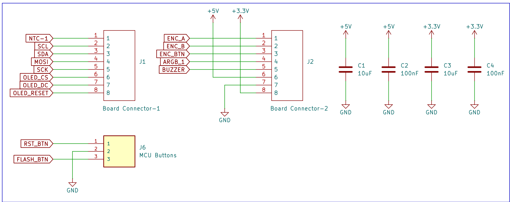
Motherboard/System Controller Connectors
