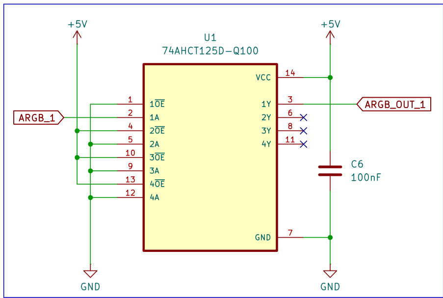
Logic Level Shifter
