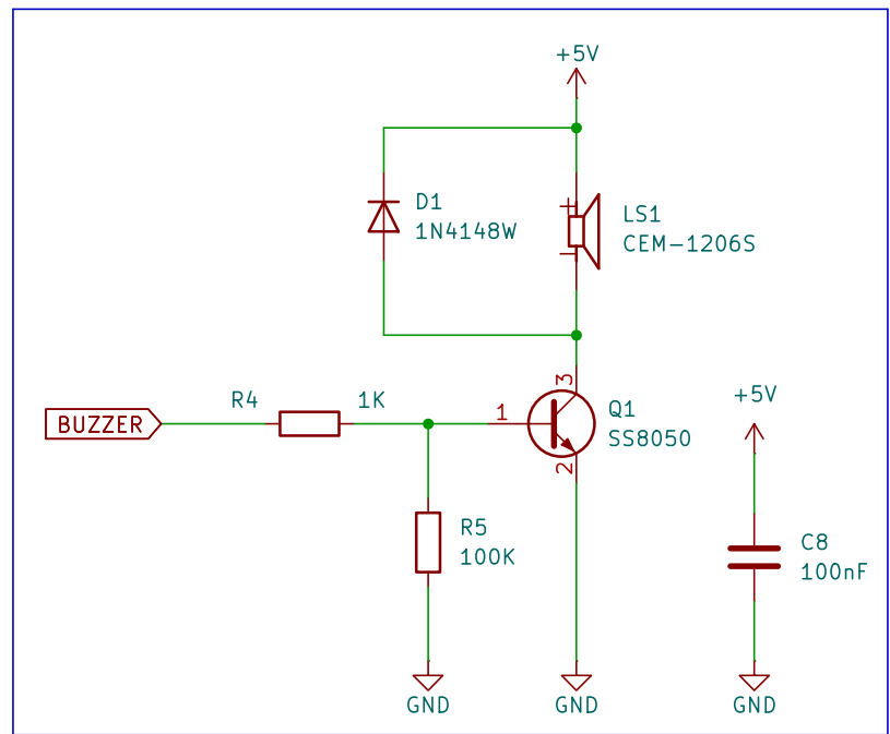
System Buzzer
