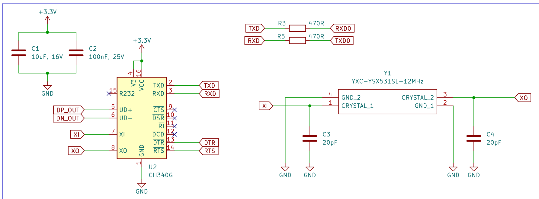
USB to UART Bridge Circuit (Option-2)
