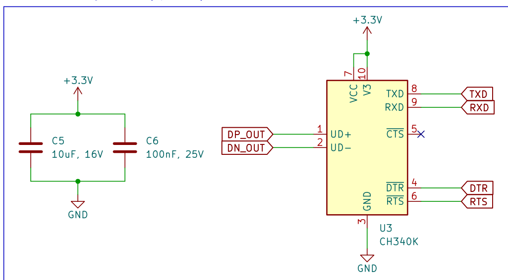
USB to UART Bridge Circuit (Option-1)
