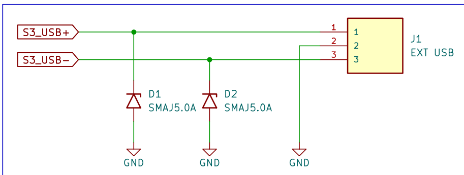
External USB Module Connector
