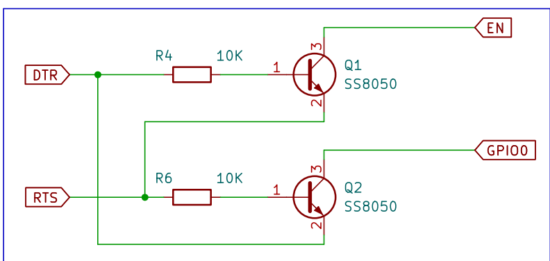
ESP32 MCU Auto Programming Circuit
