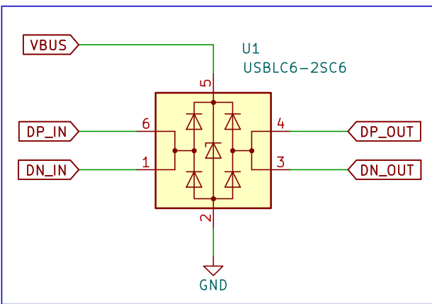
ESD Protection Circuit
