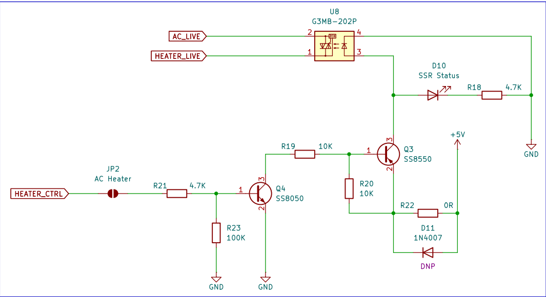
220VAC PTC Heating Element Control (Active-Low SSR, Active-High Signal)
