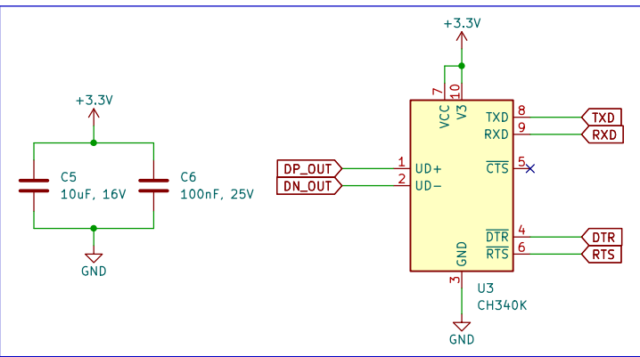
USB to UART Bridge Circuit (Option-1)
