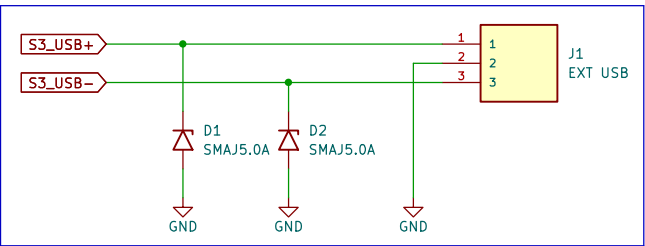
External USB Module Connector
