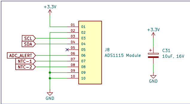
ADS1115 16-bit ADC Module Connector
