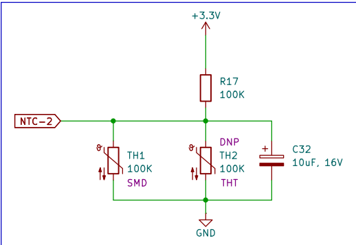
NTC Ambient Temp Sensor (Controller Board)
