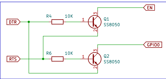
ESP32 MCU Auto Programming Circuit
