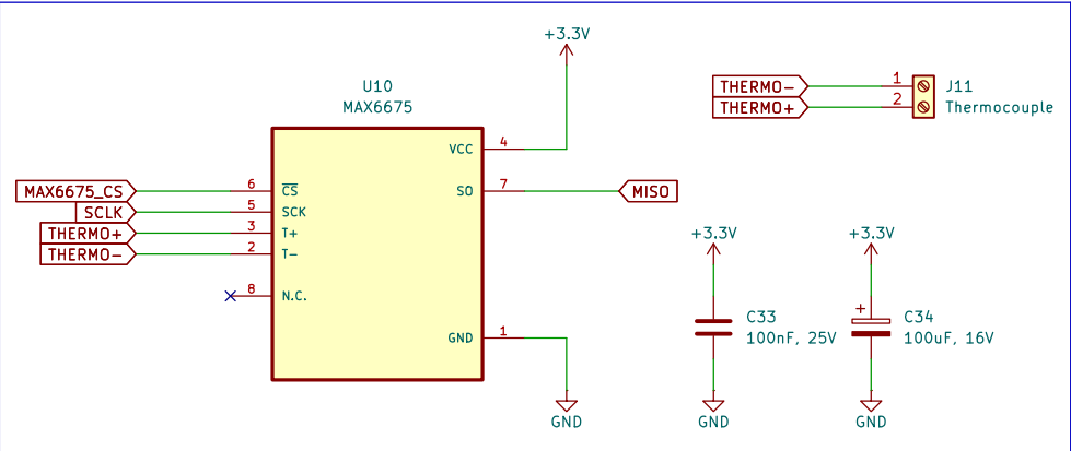
Hot Plate Temperature Sensor (K-Type Thermocouple)
