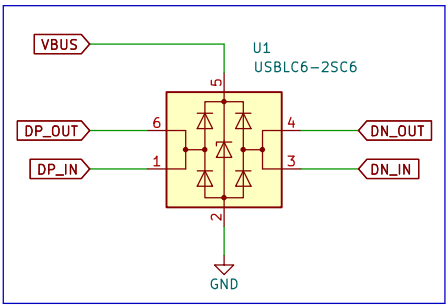
ESD Protection Circuit
