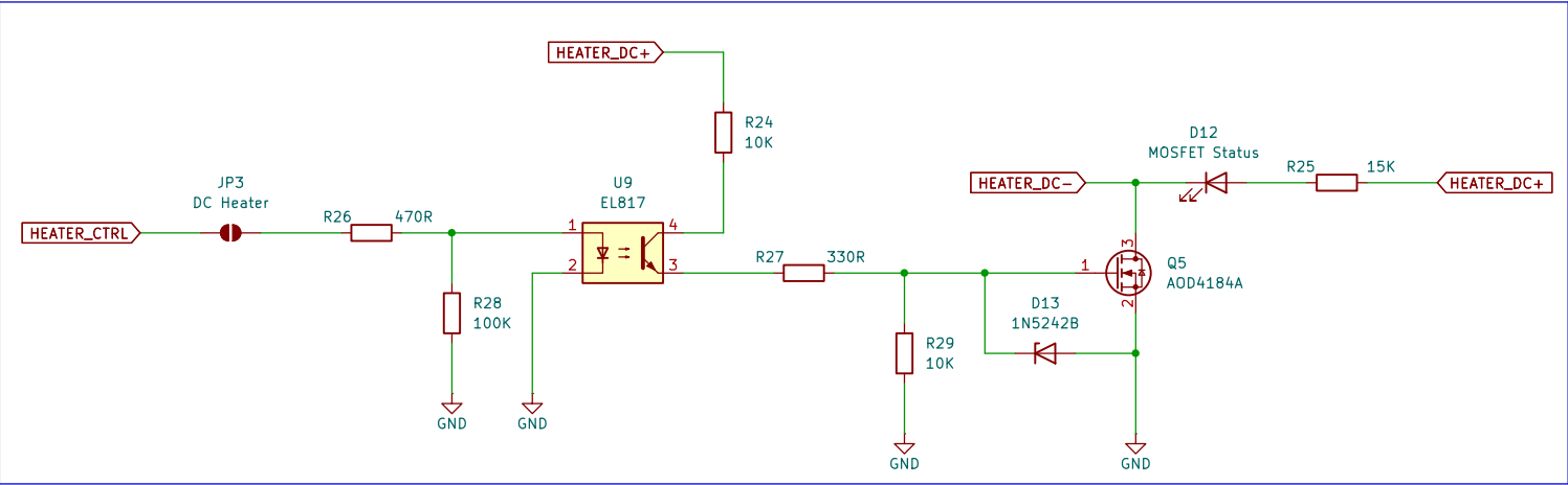
DC PTC Heating Element Control (Low-Side MOSFET Switch)
