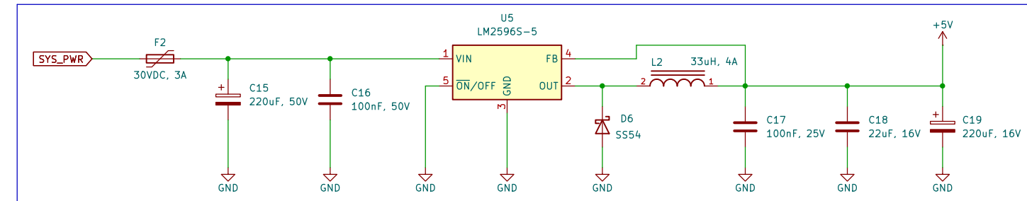
5V, 3A Step-Down Regulator/Buck Converter
