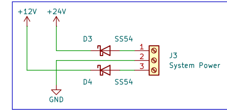
System Power Connector
