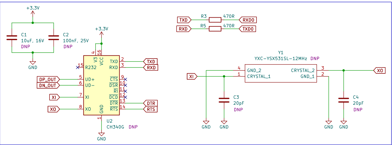
USB to UART Bridge Circuit (Option-2)
