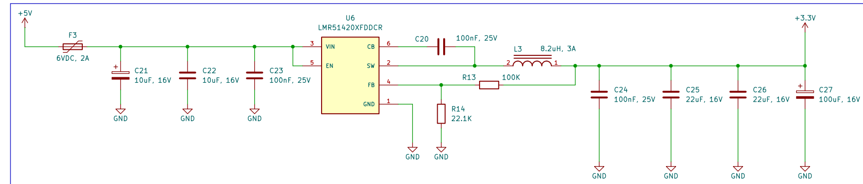
3.3V, 2A Buck Converter (MCU Power + Peripherals Power)
