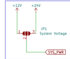
System Power Voltage Selection Jumper
