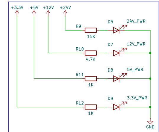
System Power LED Indicators
