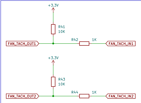
Fan Tachometer Read Circuit
