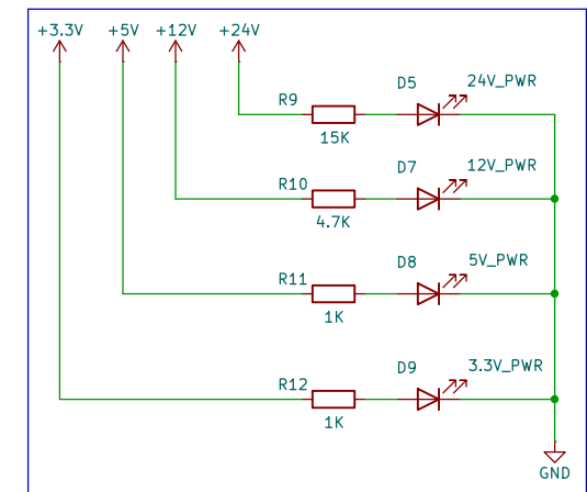
System Power LED Indicators
