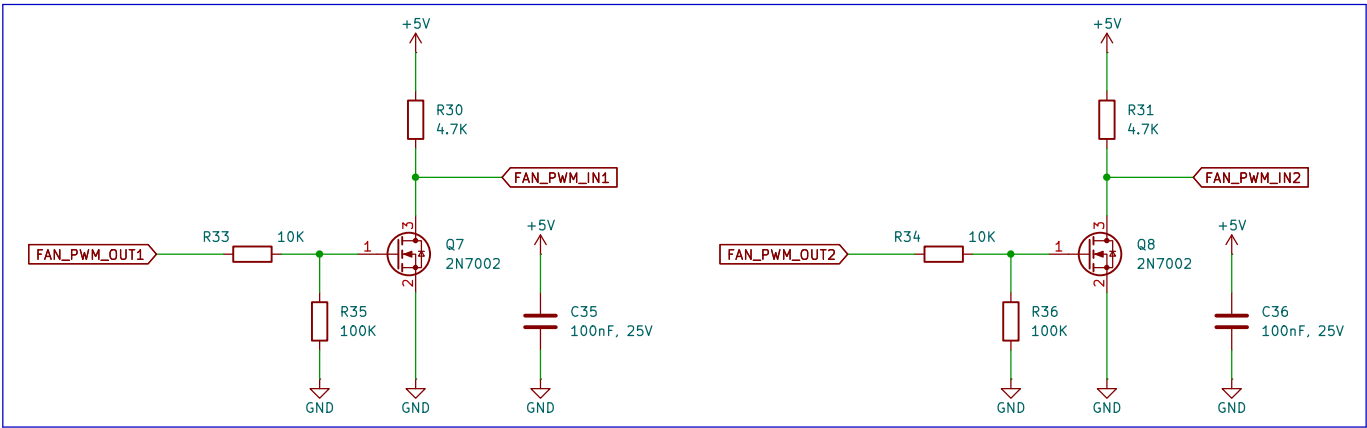
N-MOSFET Open-Drain Level Shifter / PWM Distribution Buffer
