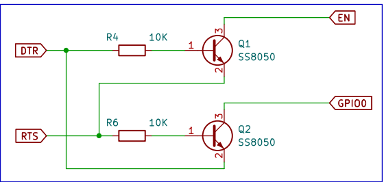
ESP32 MCU Auto Programming Circuit
