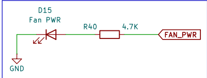
Fan Power Status LED
