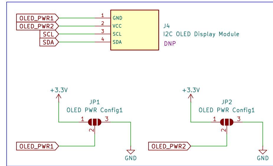
I2C OLED Display Module Connector with configurable Power Input (Option-2)
