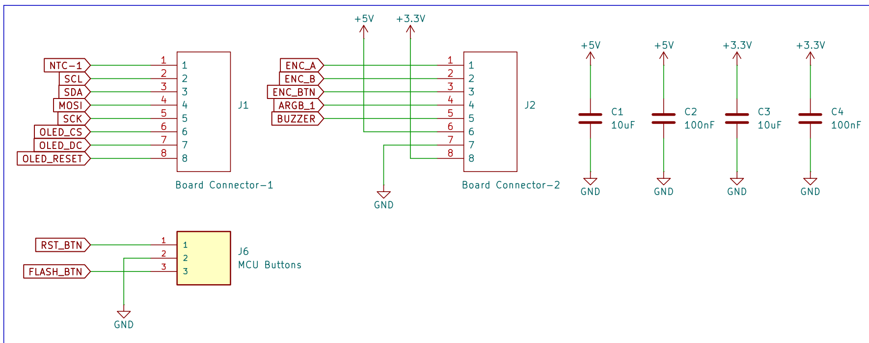
Motherboard/System Controller Connectors
