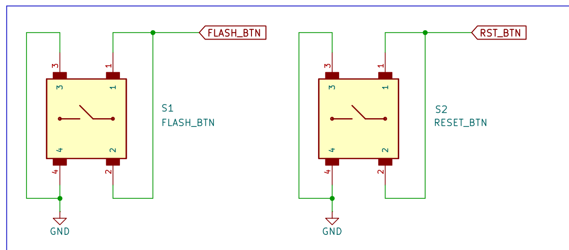
Main Board Flash and Reset Buttons
