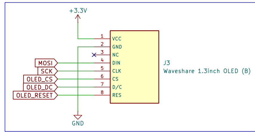
SPI OLED Display Module Connector (Option-1)
