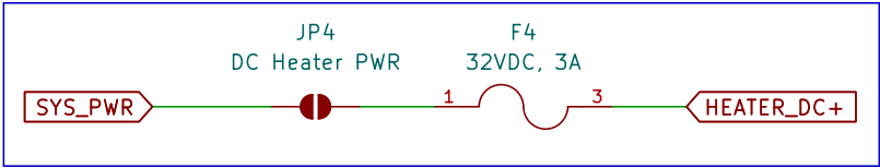
DC PTC Heating Element Power Enable Jumper
