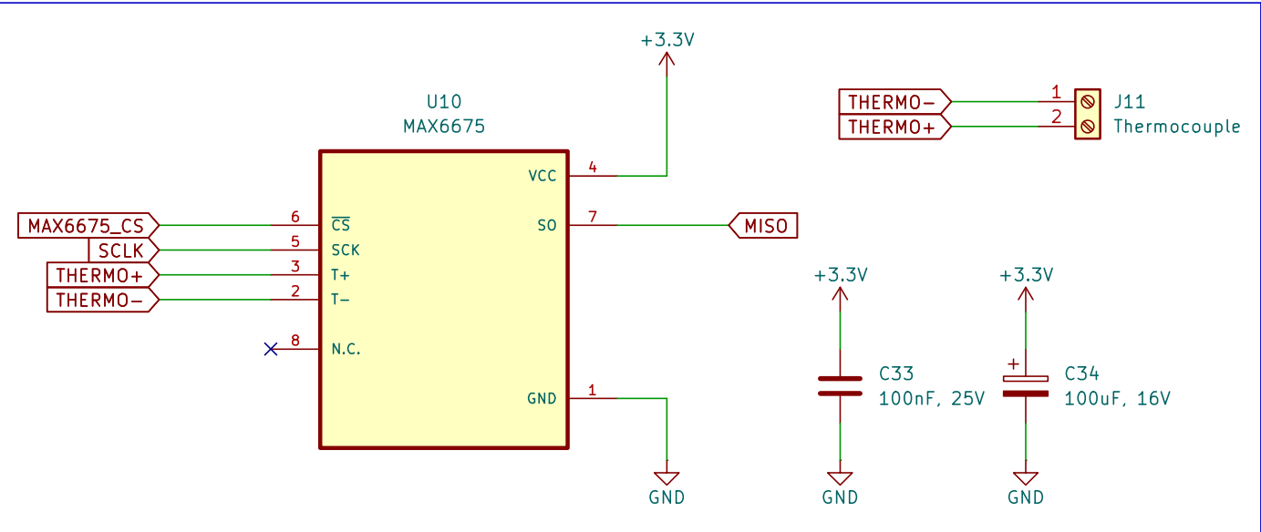
Hot Plate Temperature Sensor (K-Type Thermocouple)
