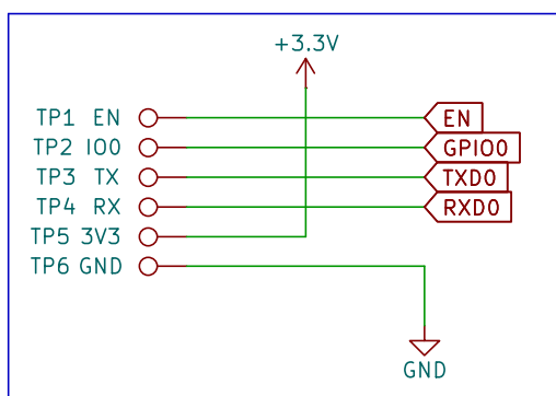
UART Test Pads
