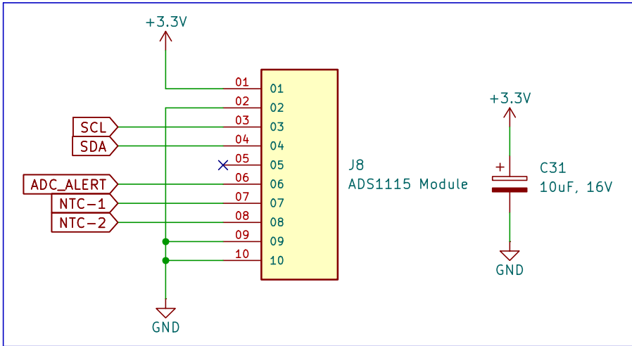
ADS1115 16-bit ADC Module Connector
