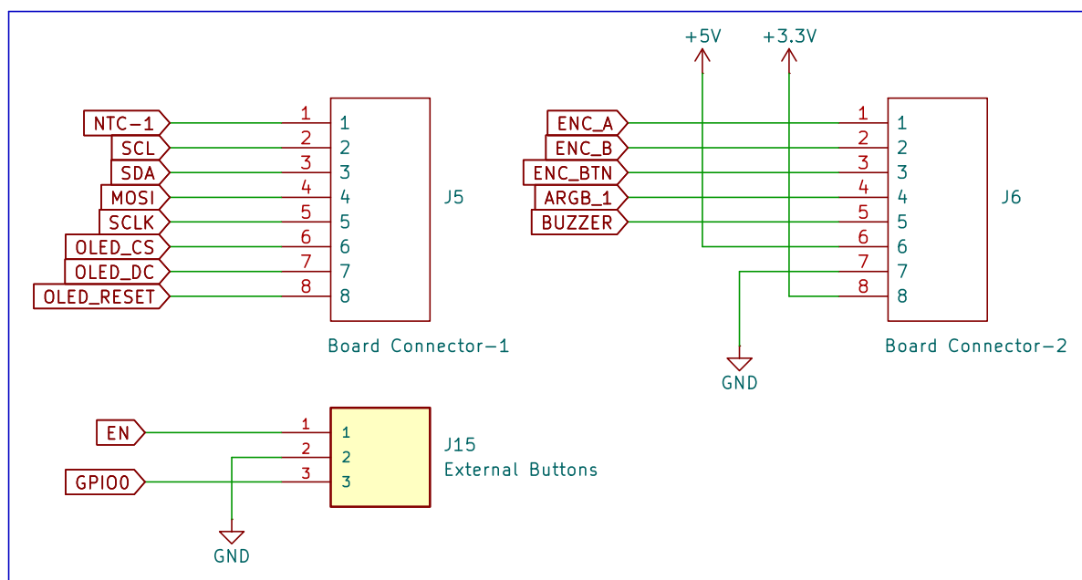
DaughterBoard (User Interface Board) Connectors
