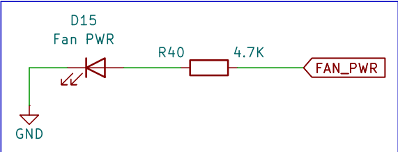
Fan Power Status LED
