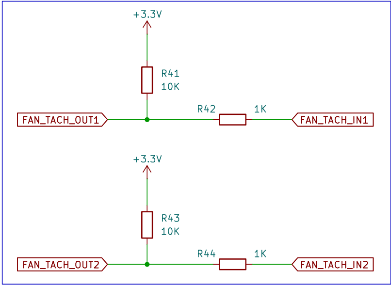
Fan Tachometer Read Circuit
