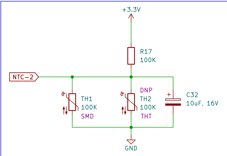
NTC Ambient Temp Sensor (Controller Board)
