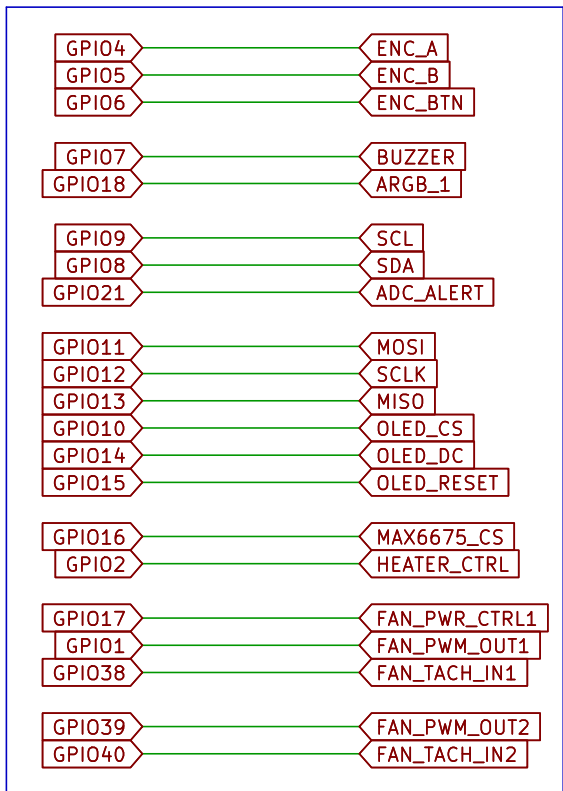
MCU GPIO Pins Allocation/Configuration
