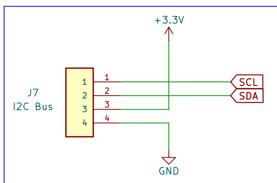
I2C Bus Connector
