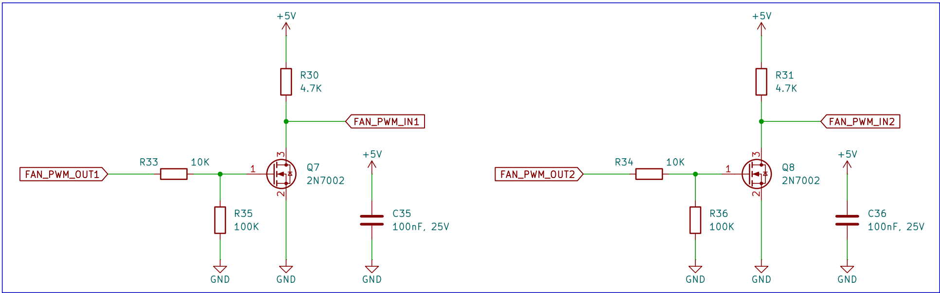
N-MOSFET Open-Drain Level Shifter / PWM Distribution Buffer
