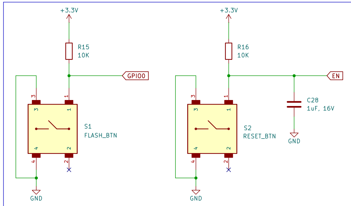
MCU Flash and Reset Buttons
