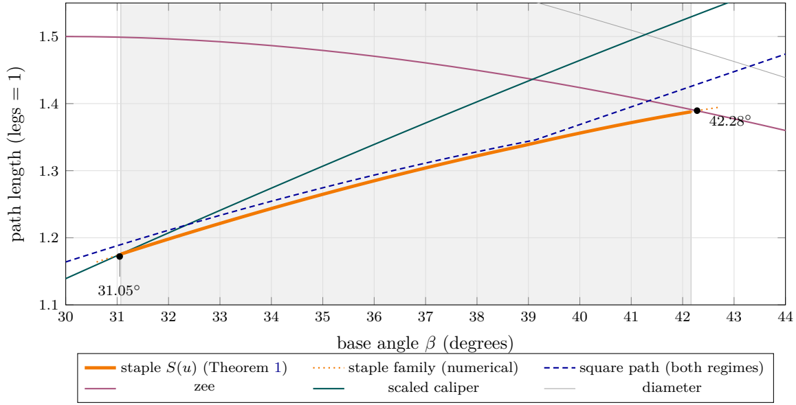
FIGURE 1. The five candidate lengths against the base angle \beta . The shaded band [31.07^\circ, 42.16^\circ] is the certified domain of Theorem 1: there the staple S(u) (thick) escapes and lies strictly below the square-path curve, whose two regimes meet in the visible kink at \beta_0 = 39.132^\circ . On [31.50^\circ, 42.16^\circ] it lies below all four competitors (Corollary 2). Dotted continuations and the two crossing points at 31.05^\circ and 42.28^\circ are numerical (Section 5); everything else in the band is proved.
