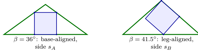
FIGURE 5. The two inscribed squares behind Lemma 9. Left: the base-aligned square, with both bottom corners on the base and both top corners on the legs. Right: the leg-aligned square, with one full side on a leg, its far corner at the apex, and one corner on the base (contacts marked). Any escaping square path must have side at least \max(s_A, s_B) ; the certificates prove |S(u)| < 3s_A for u \leq 0.365 and |S(u)| < 3s_B for u \geq 0.36 , which together cover the whole interval.
