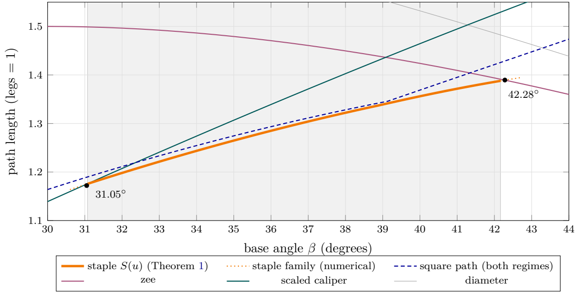
FIGURE 3. The five candidate lengths against the base angle \beta . The shaded band [31.07^\circ, 42.16^\circ] is the certified domain of Theorem 1: there the staple S(u) (thick) escapes and lies strictly below the square-path curve, whose two regimes meet in the visible kink at \beta_0 = 39.132^\circ . On [31.50^\circ, 42.16^\circ] it lies below all four competitors (Corollary 2). Dotted continuations and the two crossing points at 31.05^\circ and 42.28^\circ are numerical (Section 6); everything else in the band is proved.
