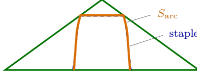
FIGURE 8. The line-arc witness S_{\text{arc}} (solid) at its critical placement in the golden gnomon, against the polygonal staple of Theorem 3 (dashed). The shoulders bend along circular arcs of radius r \approx \sin 36^\circ ; the saving is 2.28 \times 10^{-3} .
