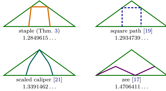
FIGURE 4. The four candidates at the golden gnomon (legs 1, apex 108^\circ , diameter 1.6180340), each drawn at a critical placement: each path's hull fits T only in touching position. The staple, square path, and caliper all touch the base with their endpoints; the caliper's peak sits exactly at the apex. The staple of Theorem 3 achieves criticality at the smallest length.
