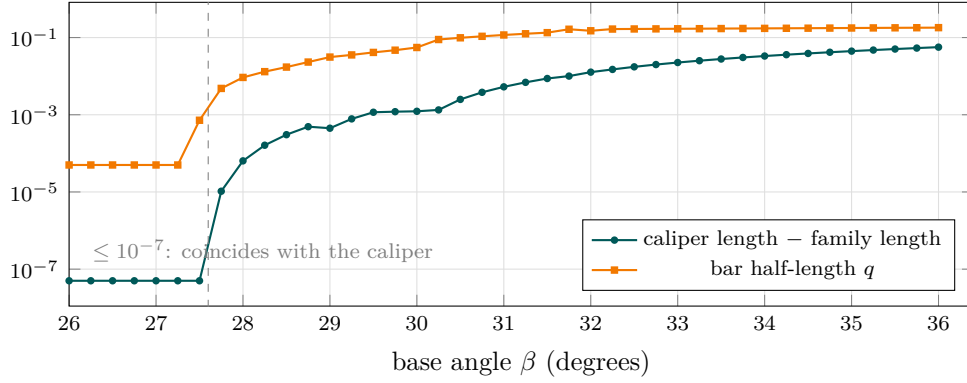
FIGURE 10. Convergence of the line-arc family onto the scaled caliper (numerical; log scale). Both the improvement over the caliper and the bar length vanish at \beta^* \approx 27.6^\circ ; clipped values at the floor of the plot are exact coincidence to solver precision.
