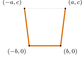
FIGURE 2. A staple and its isosceles-trapezoidal hull: the bar from (-b, 0) to (b, 0) , two equal legs to (\pm a, c) , and the dotted top edge completing the hull.
