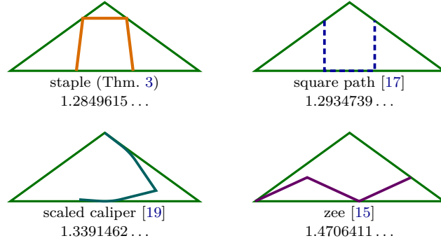
FIGURE 2. The four candidates at the golden gnomon (legs 1, apex 108^\circ , diameter 1.6180340), each drawn at a critical placement: each path's hull fits T only in touching position. The staple of Theorem 3 achieves criticality at the smallest length.
