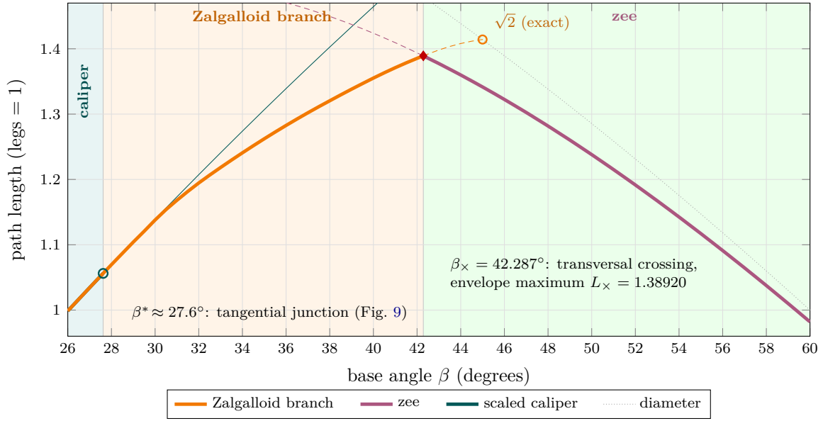
FIGURE 1. The three regimes of best-known escape paths (legs = 1): the scaled caliper for \beta \leq \beta^* \approx 27.6^\circ , the Zalgalloid line–arc branch on [\beta^*, \beta_\times] , and the zee beyond \beta_\times = 42.287^\circ . Thick curves are the frontier; dashed curves continue each branch past its regime, where it persists as a local optimum. The crossing at \beta_\times is transversal, and the kink is the maximum of the envelope: the hardest isosceles forest sits at the regime boundary (diamond). At \beta^* the branch instead merges tangentially into the caliper (circle). The branch terminates above in an exact rectangle path of length \sqrt{2} at \beta = 45^\circ (Proposition 6.3), tied with the diameter. Regime boundaries and dashed data are numerical (Sections 3.1 and 7); the zee is proven optimal on [45^\circ, 60^\circ] [5, 17]; Theorems 4.1 and 6.1 certify anchors inside the middle regime.
