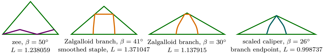
FIGURE 2. One escape path per regime, each at a critical placement in its triangle T(\beta) (legs = 1; the hull fits only in touching position). Left: the zee at \beta = 50^\circ — diagonal type, the middle segment crosses the hull. The other three panels are members of the single Zalgalloid branch — boundary type, the path traverses its hull boundary minus a chord: at 41^\circ a smoothed staple (bar under the apex, shoulder arcs of radius \sin \beta and span 3.5^\circ , to the eye still a trapezoid); at 30^\circ a deeper member (long arcs, short bar); at 26^\circ the branch's lower endpoint, the scaled caliper (bar length zero). Lengths are the best known values at each angle; placements are computed, not sketched.
