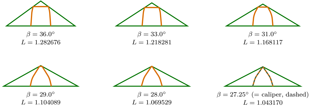
FIGURE 8. The Zalgallod family (numerical): optimized line-arc members at six base angles, each at its critical placement (tips on the base, bar or peak under the apex). As \beta decreases the bar shrinks and the arcs deepen; at \beta = 27.25^\circ the optimized member coincides with the scaled Zalgaller caliper (dashed): the vanished bar has become the caliper's peak corner, the shoulder arcs its arcs (span \tilde{\beta} = 18.27^\circ ), the tips its feet.
