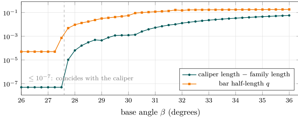
FIGURE 9. Convergence of the line-arc family onto the scaled caliper (numerical; log scale). Both the improvement over the caliper and the bar length vanish at \beta^* \approx 27.6^\circ ; clipped values at the floor of the plot are exact coincidence to solver precision.
