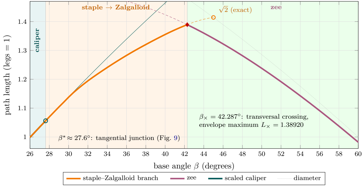
FIGURE 1. The three regimes of best-known escape paths (legs = 1): the scaled caliper for \beta \leq \beta^* \approx 27.6^\circ , the staple-to-Zalgalloid line-arc branch on [\beta^*, \beta_\times] , and the zee beyond \beta_\times = 42.287^\circ . Thick curves are the frontier; dashed curves continue each branch past its regime, where it persists as a local optimum. The crossing at \beta_\times is transversal, and the kink is the maximum of the envelope: the hardest isosceles forest sits at the regime boundary (diamond). At \beta^* the branch instead merges tangentially into the caliper (circle). The branch terminates above in an exact rectangle path of length \sqrt{2} at \beta = 45^\circ (Proposition 6.3), tied with the diameter. Regime boundaries and dashed data are numerical (Sections 3.1 and 7); the zee is proven optimal on [45^\circ, 60^\circ] [5, 17]; Theorems 4.1 and 6.1 certify anchors inside the middle regime.
