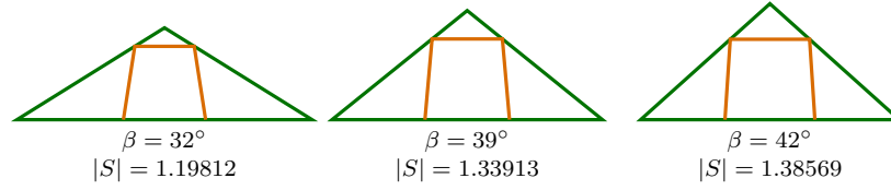
FIGURE 10. The certified family S(u) inside T(\beta) at \beta = 32^\circ, 39^\circ, 42^\circ , each at a critical placement (the hull fits only in touching position).
