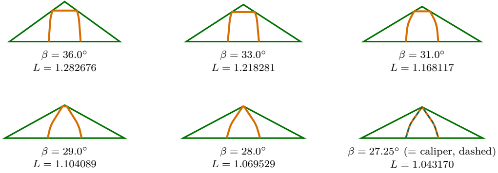
FIGURE 8. The Zalgalloid family (numerical): optimized line-arc members at six base angles, each at its critical placement (tips on the base, bar or peak under the apex). As \beta decreases the bar shrinks and the arcs deepen; at \beta = 27.25^\circ the optimized member coincides with the scaled Zalgaller caliper (dashed): the vanished bar has become the caliper's peak corner, the shoulder arcs its arcs (span \tilde{\beta} = 18.27^\circ ), the tips its feet.
