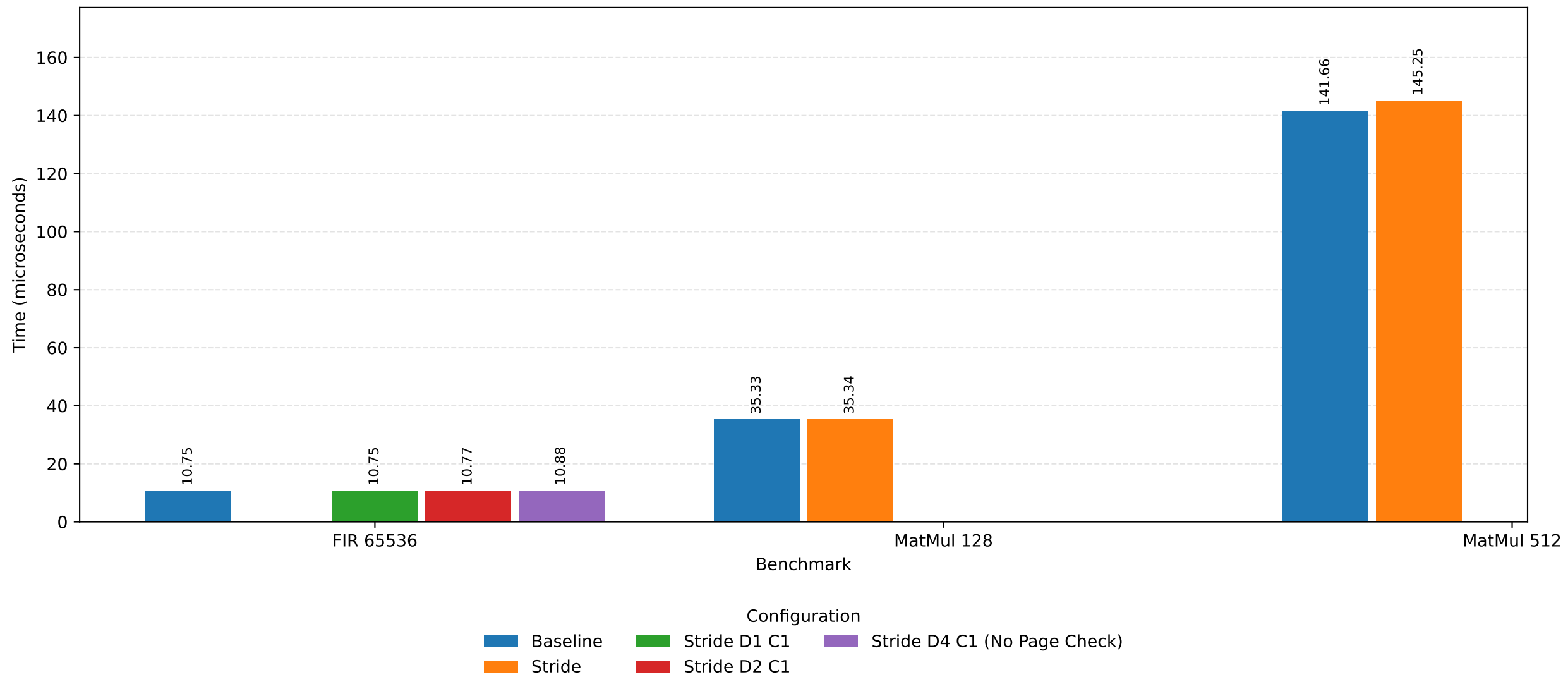
Execution Time
