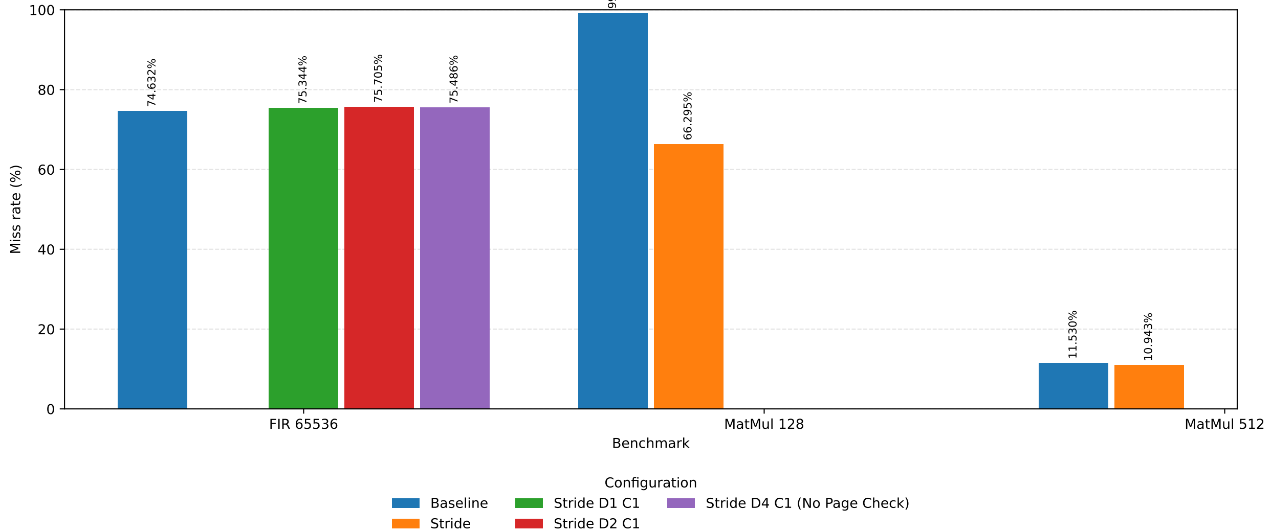
L2 Demand Cache Miss Rate
