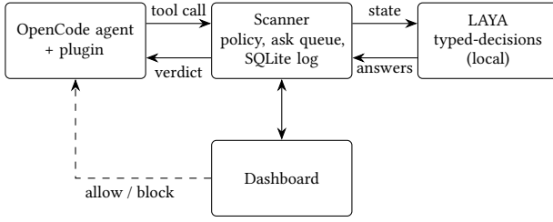
Figure 1: Secure Guard architecture. The scanner scores every tool call with LAYA before it runs. Depending on the mode, a flagged call is logged (monitor), held for the user (ask) or blocked (auto).
