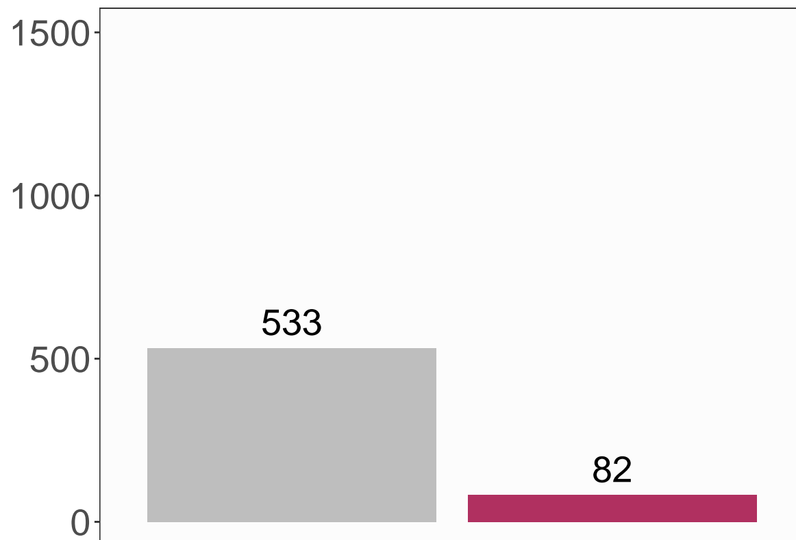
Bluehead Chub
