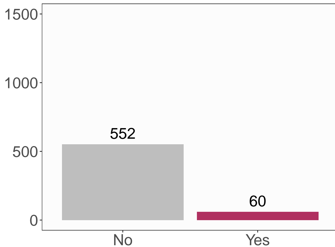
Green Sunfish
