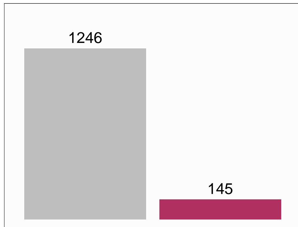
Creek Chub
