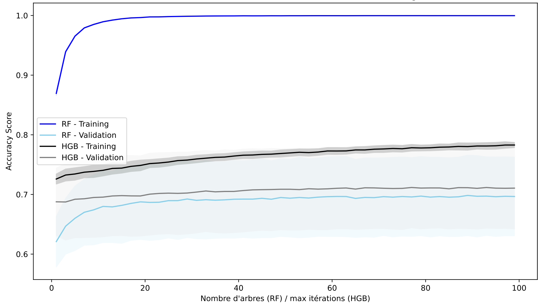
Validation Curve: Random Forest vs HistGradientBoosting
