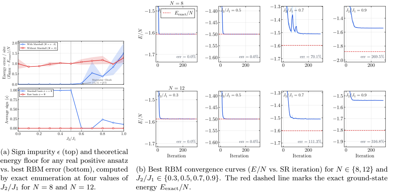
Figure 8: Visualization of the sign problem on the J_1 - J_2 Heisenberg chain. Left: sign impurity and overall training dynamics, Right: best run for selected instances.
