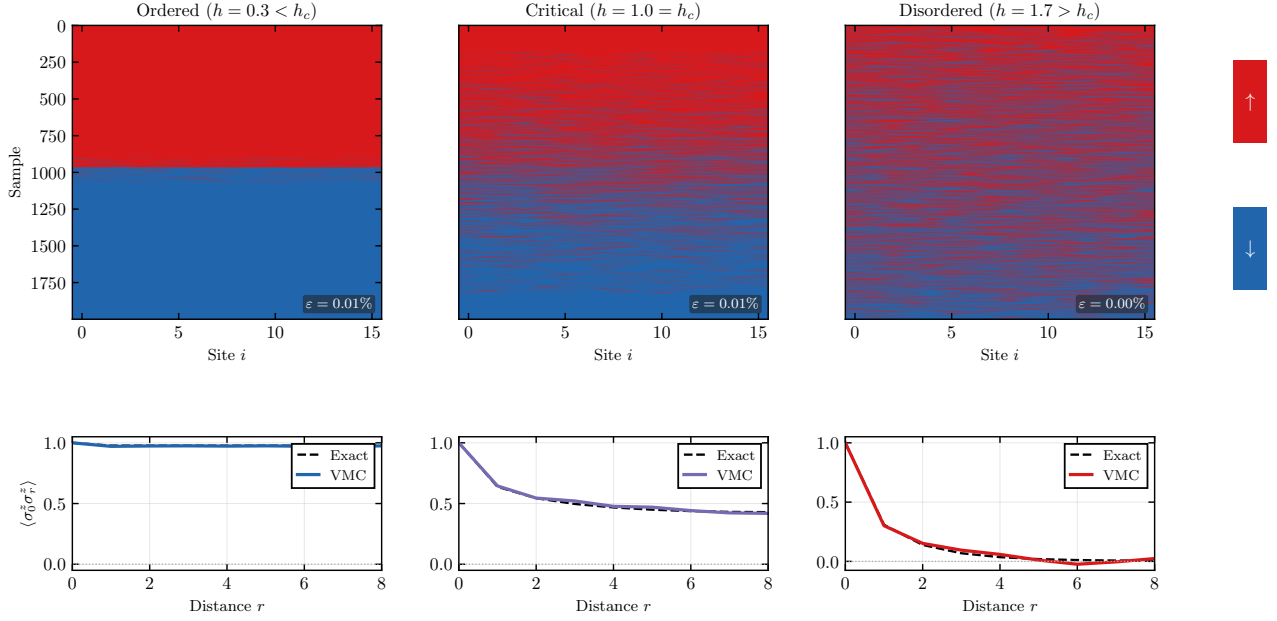
Figure 7: Spin configurations sampled from a trained RBM-VMC model for the one-dimensional Transverse-Field Ising Model (TFIM) at three values of the transverse field h . Top row: each column shows 2000 spin configurations \sigma \in \{-1, +1\}^N sampled from the learned wave function |\Psi_\theta|^2 , sorted by total magnetisation. Bottom row: spin-spin correlation C(r) = \langle \sigma_0^z \sigma_r^z \rangle as a function of distance r , computed from VMC samples (solid line) and exact diagonalisation (dashed line). The relative energy error \varepsilon = |E_{\text{VMC}} - E_{\text{exact}}|/|E_{\text{exact}}| is shown in each panel. The model is a fully-connected RBM ( N = N_h = 16 ) trained for 300 iterations of Stochastic Reconfiguration with 500 Metropolis-Hastings samples per step.
