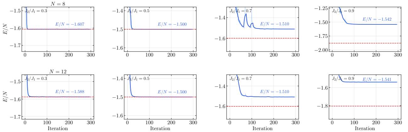
Figure 10: Best RBM convergence curves ( E/N vs. SR iteration) for N \in \{8, 12\} and J_2/J_1 \in \{0.3, 0.5, 0.7, 0.9\} on the frustrated J_1 - J_2 Heisenberg chain. The red dashed line marks the exact ground-state energy E_{\text{exact}}/N . The lowest achieved relative error increases with J_2/J_1 .
