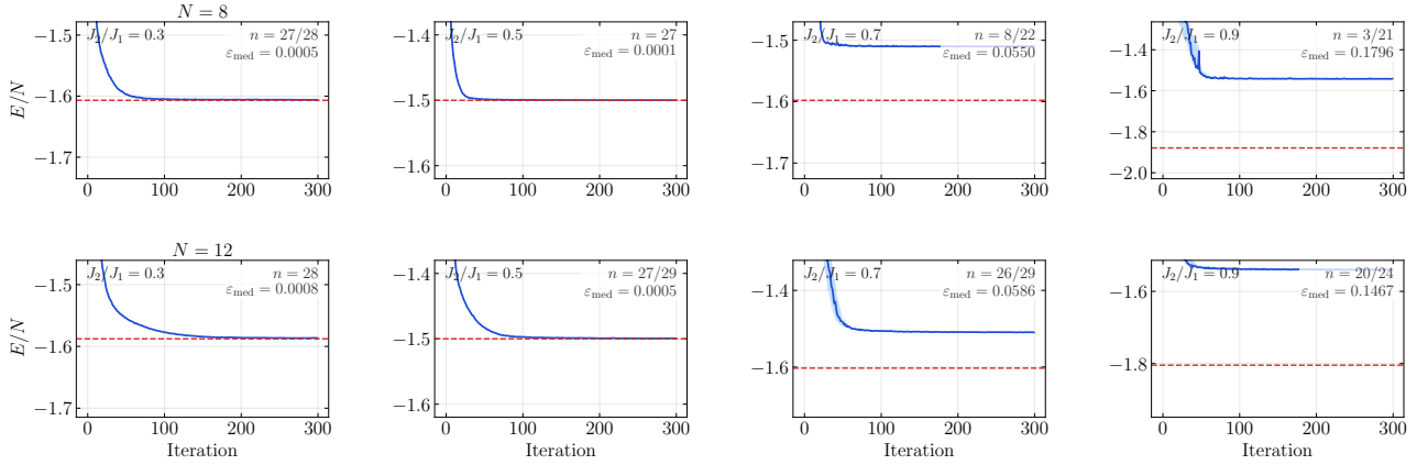
Figure 10: RBM convergence curves ( E/N vs. SR iteration) for N \in \{8, 12\} and J_2/J_1 \in \{0.3, 0.5, 0.7, 0.9\} on the frustrated J_1 - J_2 Heisenberg chain, using Gibbs sampling. The solid line is the median over n independent evaluation seeds (annotated per panel); the shaded band is the interquartile range. For each panel, the hyper-parameter configuration was selected beforehand on a disjoint tuning set (Optuna trials, tuning seeds excluded from evaluation); \varepsilon_{\text{med}} denotes the median relative error of the tail-averaged energy. Where n is reported as a/b , b seeds were attempted and b - a runs diverged (non-finite energy) under the selected configuration and are retained as failures rather than silently dropped; divergence is frequent in the strongly frustrated regime ( N = 8 , J_2/J_1 \geq 0.7 ). The red dashed line marks the exact ground-state energy E_{\text{exact}}/N . The median relative error rises sharply beyond J_2/J_1 = 0.5 .
