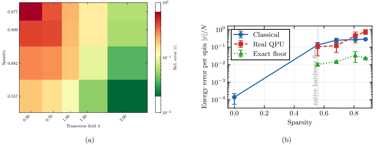
Figure 12: Error as a function of sparsity, with the number of hidden units kept equal to the number of visible units in both plots. (a) Error for different values of h . (b) Error at h = 1 , comparing classical training to training on the real QPU. The dotted line marks the exact-ansatz floor at this size.
