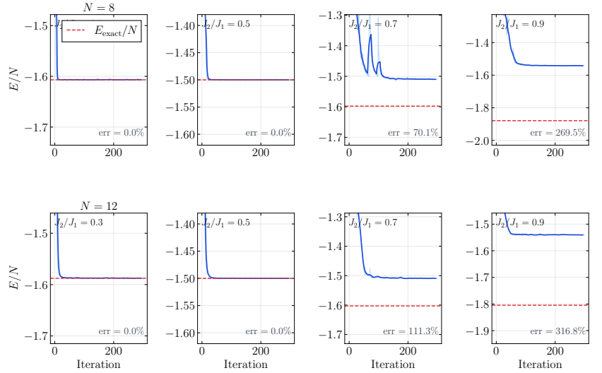
(b) Best RBM convergence curves ( E/N vs. SR iteration) for N \in \{8, 12\} and J_2/J_1 \in \{0.3, 0.5, 0.7, 0.9\} . The red dashed line marks the exact ground-state energy E_{\text{exact}}/N . Before and at the Majumdar–Ghosh point ( J_2/J_1 \leq 0.5 ) the RBM converges to the ground state (relative error 0.0%). Beyond it the optimiser stalls well above the exact energy, with the gap growing with J_2/J_1 and with system size N .
