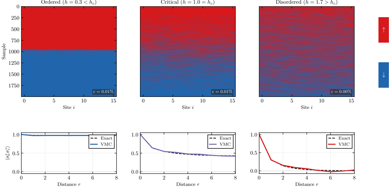
Figure 6: Spin configurations sampled from a trained RBM-VMC model for the one-dimensional Transverse-Field Ising Model (TFIM) at three values of the transverse field h . Top row: each column shows 2000 spin configurations \sigma \in \{-1, +1\}^N sampled from the learned wave function |\Psi_\theta|^2 , sorted by total magnetisation. Bottom row: spin-spin correlation C(r) = \langle \sigma_0^z \sigma_r^z \rangle as a function of distance r , computed from VMC samples (solid line) and exact diagonalisation (dashed line). The relative energy error \epsilon = |E_{\text{VMC}} - E_{\text{exact}}|/|E_{\text{exact}}| is shown in each panel. The model is a fully-connected RBM ( N = N_h = 16 ) trained for 300 iterations of Stochastic Reconfiguration with 500 Metropolis-Hastings samples per step.
