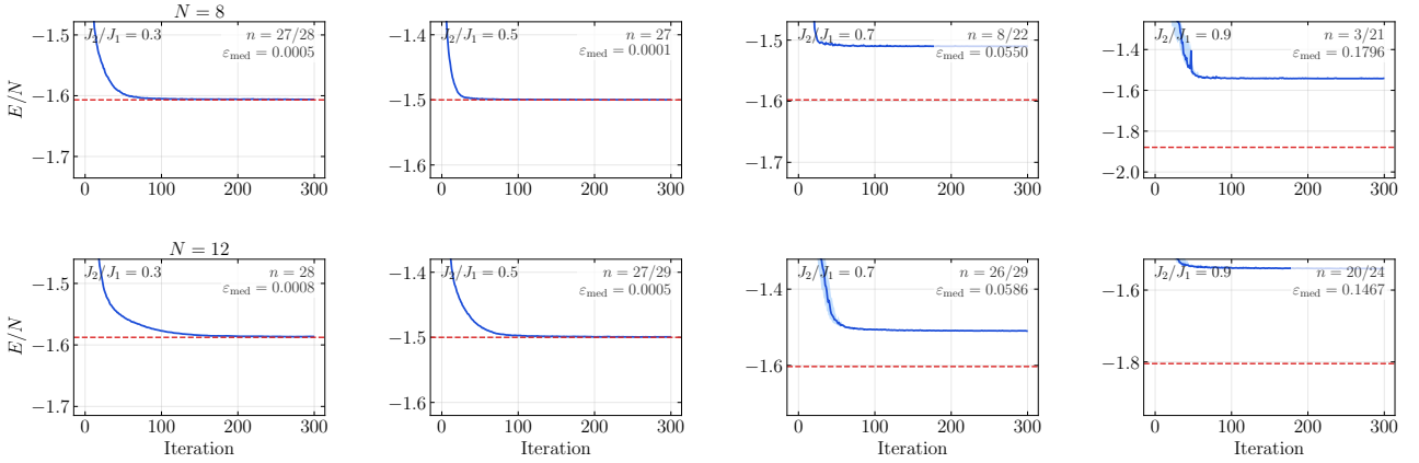
Figure 11: RBM convergence curves ( E/N vs. SR iteration) for N \in \{8, 12\} and J_2/J_1 \in \{0.3, 0.5, 0.7, 0.9\} on the frustrated J_1 - J_2 Heisenberg chain, using Gibbs sampling. The solid line is the median over n independent evaluation seeds (annotated per panel); the shaded band is the interquartile range. For each panel, the hyper-parameter configuration was selected beforehand on a disjoint tuning set (Optuna trials, tuning seeds excluded from evaluation); \varepsilon_{\text{med}} denotes the median relative error of the tail-averaged energy. Where n is reported as a/b , b seeds were attempted and b - a runs diverged (non-finite energy) under the selected configuration and are retained as failures rather than silently dropped; divergence is frequent in the strongly frustrated regime ( N = 8 , J_2/J_1 \geq 0.7 ). The red dashed line marks the exact ground-state energy E_{\text{exact}}/N . The median relative error rises sharply beyond J_2/J_1 = 0.5 .
