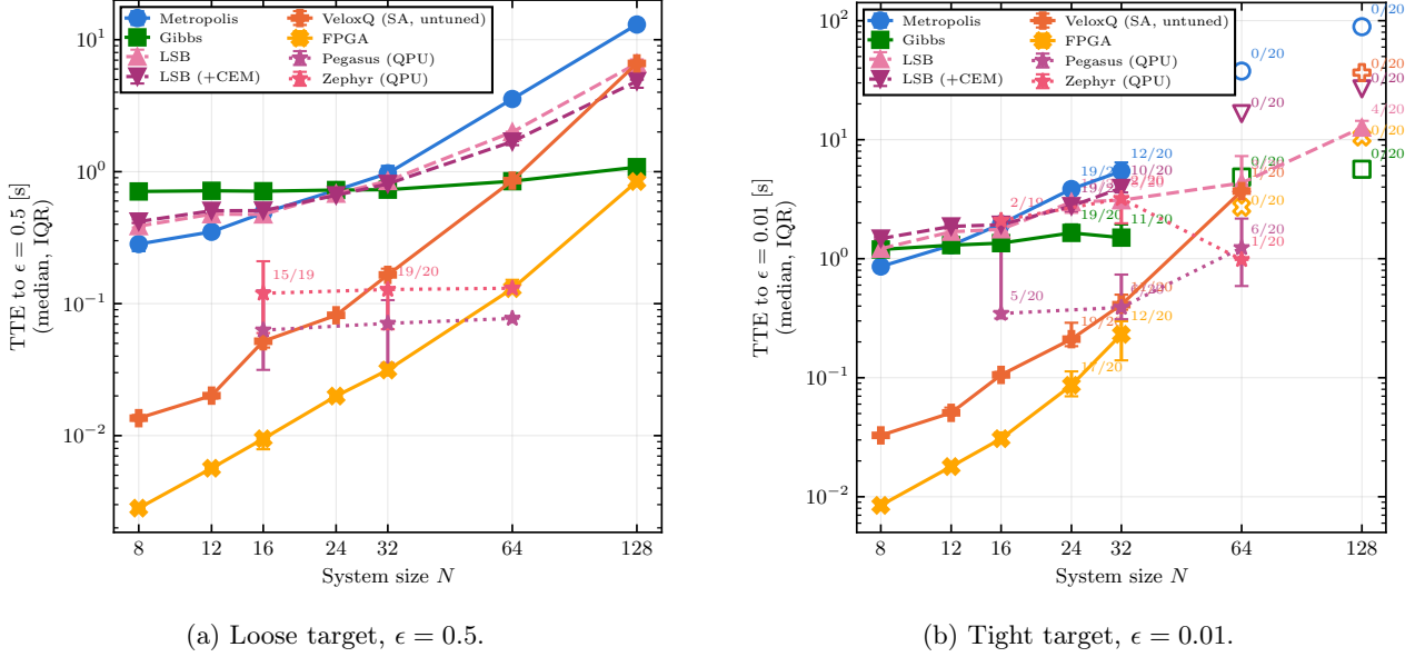
Figure 6: Time-to- \epsilon (TTE) versus system size N , all solvers, for the one-dimensional TFIM at h = 0.5 with N_h = N . Every series uses matched hyperparameters (learning rate 0.08, regularization 0.05, 200 samples per iteration, 100 iterations); markers show the median over up to 20 seeds with the interquartile range, hollow markers mark sizes where at least one seed was censored (never reached \epsilon ), annotated with the fraction of seeds that reached threshold. QPU (Pegasus, Zephyr) results are shown for N \in \{16, 32, 64\} only. (a) Loose accuracy target. (b) Tight accuracy target.
