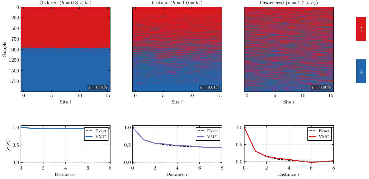
Figure 10: Spin configurations sampled from a trained RBM-VMC model for the one-dimensional Transverse-Field Ising Model (TFIM) at three values of the transverse field h . Top row: each column shows 2000 spin configurations \sigma \in \{-1, +1\}^N sampled from the learned wave function |\Psi_\theta|^2 , sorted by total magnetisation. Bottom row: spin-spin correlation C(r) = \langle \sigma_0^z \sigma_r^z \rangle as a function of distance r , computed from VMC samples (solid line) and exact diagonalisation (dashed line). The relative energy error \varepsilon = |E_{\text{VMC}} - E_{\text{exact}}|/|E_{\text{exact}}| is shown in each panel. The model is a fully-connected RBM ( N = N_h = 16 ) trained for 300 iterations of Stochastic Reconfiguration with 500 Metropolis-Hastings samples per step.
