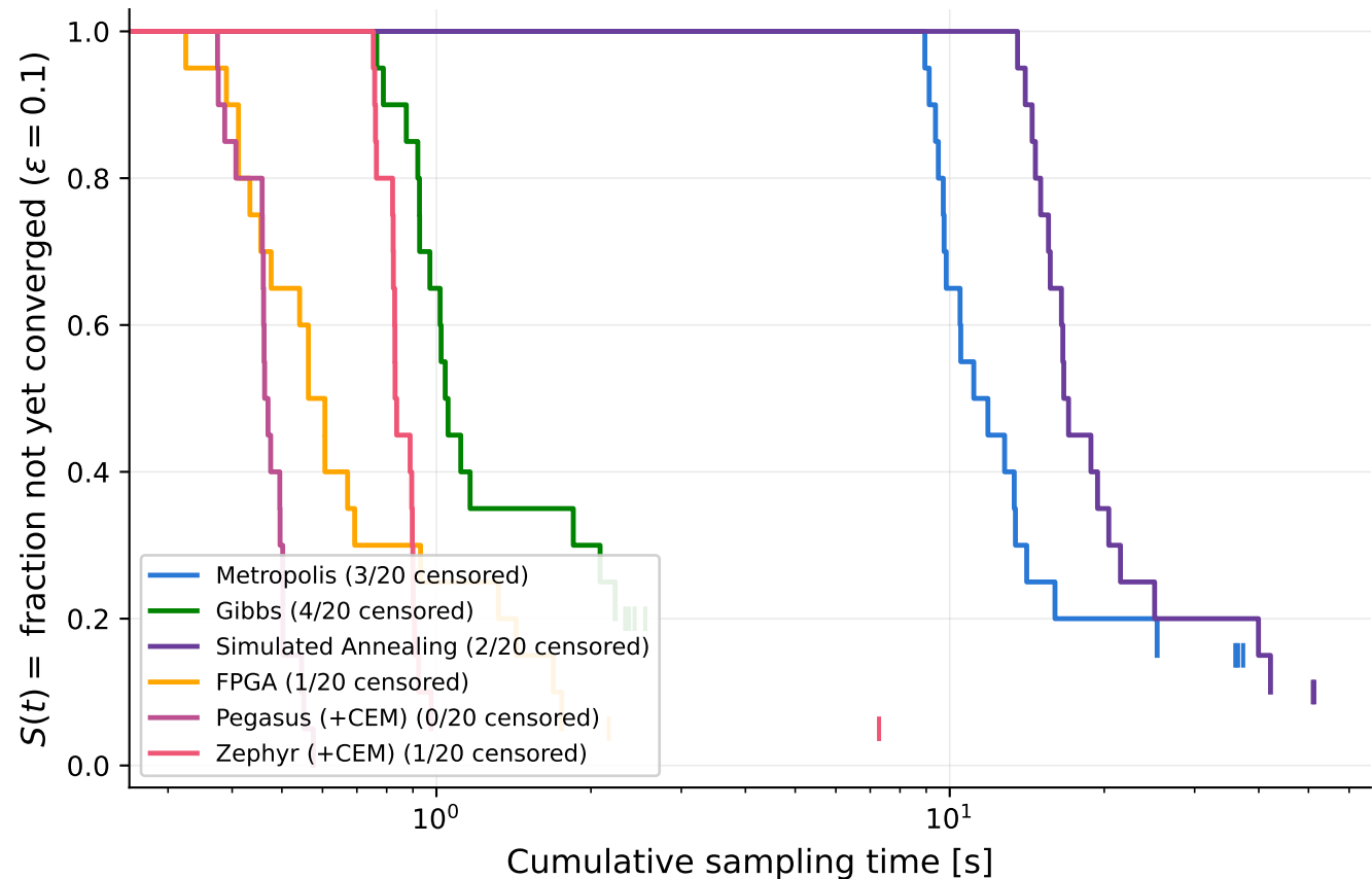
Kaplan-Meier convergence curves, N = 64 , h = 0.5 (tick = censored seed, i.e. did not converge in budget)
