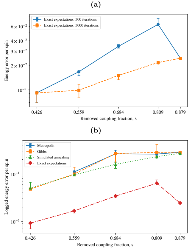
FIG. 9. (a) Exact-expectation training at 300 vs. 3000 iterations across sparsity masks. (b) Matched-iteration (300) comparison of exact expectations against three classical samplers. Five seeds per point; markers are medians, bars span first/third quartiles.
