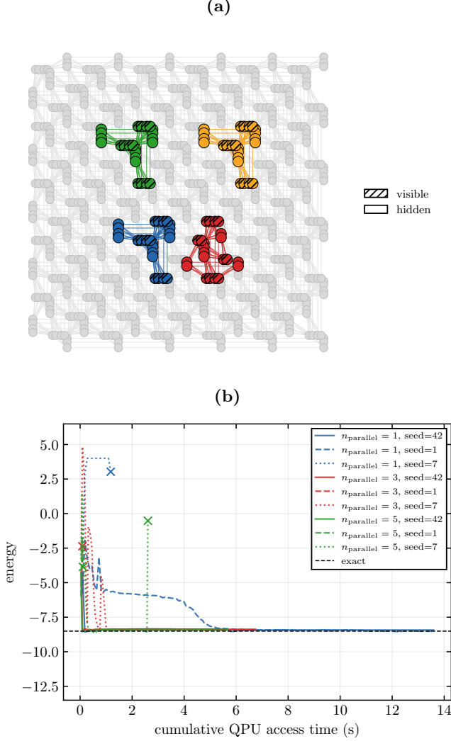
FIG. 10. (a) A four-copy Pegasus embedding layout. (b) All nine recorded training trajectories vs. cumulative QPU access time; crosses mark divergence.
