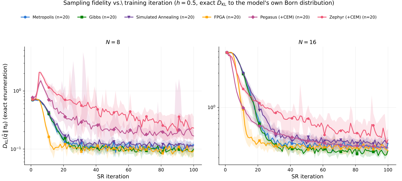
FIG. 3. Exact D_{\text{KL}}(\hat{q}||\pi_\theta) vs. SR iteration, h = 0.5 , N = 8, 16 (median and IQR band, 20 seeds per solver). Classical MCMC (Metropolis, Gibbs, simulated annealing) and FPGA converge to a common, tight floor by iteration \sim 20 –30. Pegasus(+CEM) and Zephyr(+CEM) settle above that floor, with visibly wider bands – a directly quantified, exact-enumeration version of the “residual non-Gibbs distortion” this section otherwise only measures indirectly through D_{\text{TV}} at one instance. All curves start high and decline: the RBM’s own Born distribution is close to unstructured at initialization, and concentrates onto a lower-entropy manifold as SR training proceeds, which is mechanically easier for a finite sample to resolve regardless of sampler – confirmed by Metropolis, whose \beta_x is fixed at exactly 1 throughout and shows the same decline. Pegasus(+CEM) and Zephyr(+CEM) additionally show an early rise before falling; we checked and ruled out a simple explanation (their \beta_x is already fluctuating in its eventual steady range during this rise, not still converging from a poorly calibrated start), so the mechanism behind the hump is left as an open question rather than asserted.
