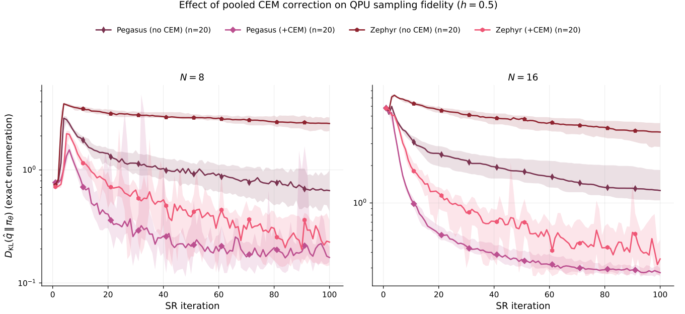
FIG. 4. Effect of pooled CEM correction on exact D_{\text{KL}}(\hat{q}||\pi_\theta) , h = 0.5 , N = 8, 16 (median and IQR band, 20 seeds per arm). cem=0 (uncorrected) sits nearly an order of magnitude above cem=1 throughout training for both devices, with the larger benefit for Zephyr. This is direct evidence that the pooled-CEM estimator of Sec. II B improves the sampled distribution itself, not only the logged training energy – the empirical counterpart to the theoretical properties left open in Sec. II E.
