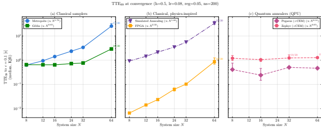
FIG. 8. TTE_{99} (Eq. (12)) vs. N at the single tested cell h = 0.5 , \epsilon = 0.1 . Annotated fractions give the successful-seed count where below 20/20. This is the only (\epsilon, h) cell for which a full- N curve currently exists; Sec. VB explains why it should not be read as representative.
