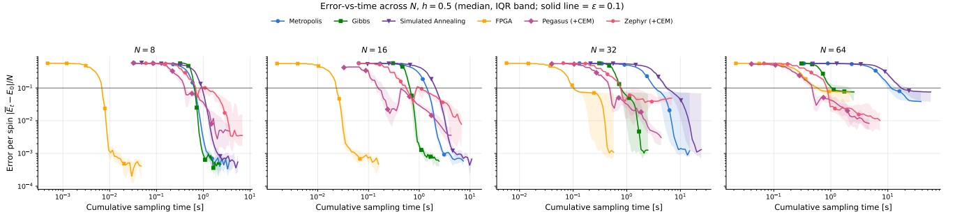
FIG. 7. Achieved energy error per spin vs. cumulative sampling time, h = 0.5 , N = 8, 16, 32, 64 (median and IQR band, 20 seeds per solver per size). Horizontal line marks \epsilon = 0.1 . At N = 64 , the median curves for Pegasus(+CEM), FPGA, and Zephyr(+CEM) cross \epsilon = 0.1 within a factor of \sim 2 of each other (0.47 s, 0.59 s, 0.84 s respectively) with visibly overlapping IQR bands, while Metropolis and simulated annealing cross more than an order of magnitude later (11.5 s, 17.1 s). Reanalysis script and both formats archived at figures/reanalysis/reanalyze_tte.py .
