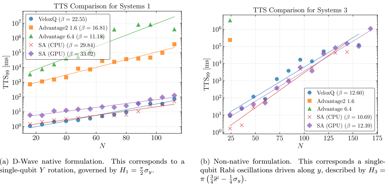
Figure 1: Previous work on sampling the exact ground state to simulate quantum systems. TTS 99 vs. N : exponential scaling \propto \exp(N/\beta) . GPU solvers dominate for N \gtrsim 100 ; missing points indicate zero success probability.
