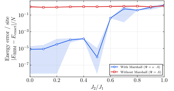
FIG. 12. Heisenberg energy error per spin, positive-amplitude vs. fixed-Marshall-sign ansatz, N = 8 , three seeds. Bands are recorded standard deviations.
