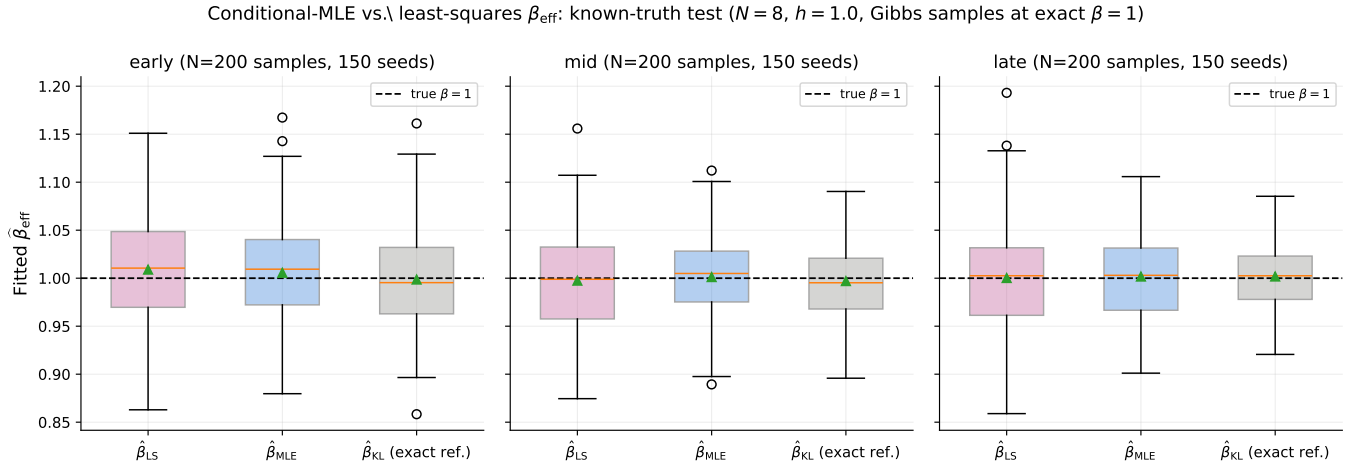
FIG. 9. \hat{\beta}_{\text{LS}} , \hat{\beta}_{\text{MLE}} , and the exact-enumeration reference \hat{\beta}_{\text{KL}} , fit to 150 independent fresh Gibbs samples per training stage from the three surviving cem_validation_sweep.py checkpoints ( N = 8 , h = 1.0 ). The true generating \beta is exactly 1 (dashed line) by construction of the sampler, not merely estimated. Both conditional estimators are essentially unbiased; \hat{\beta}_{\text{MLE}} 's interquartile range is visibly narrower than \hat{\beta}_{\text{LS}} 's at the “mid” and “late” stages.
