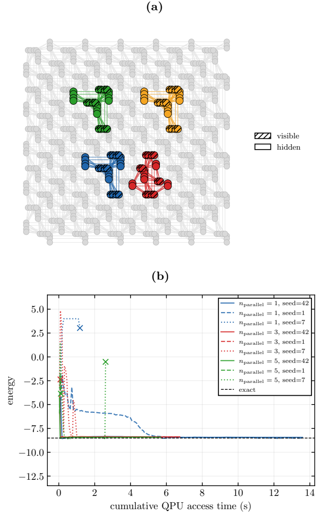
FIG. 11. (a) A four-copy Pegasus embedding layout. (b) All nine recorded training trajectories vs. cumulative QPU access time; crosses mark divergence.
