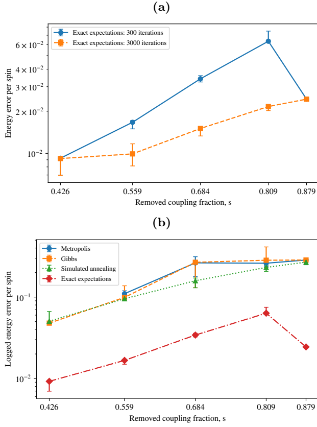
FIG. 10. (a) Exact-expectation training at 300 vs. 3000 iterations across sparsity masks. (b) Matched-iteration (300) comparison of exact expectations against three classical samplers. Five seeds per point; markers are medians, bars span first/third quartiles.
