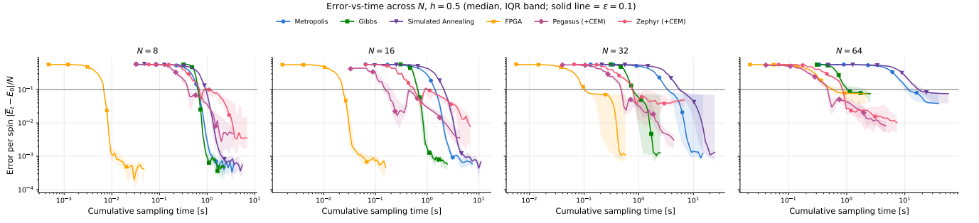
FIG. 5. Achieved energy error per spin vs. cumulative sampling time, h = 0.5 , N = 8, 16, 32, 64 (median and IQR band, 20 seeds per solver per size). Horizontal line marks \epsilon = 0.1 . At N = 64 , the median curves for Pegasus(+CEM), FPGA, and Zephyr(+CEM) cross \epsilon = 0.1 within a factor of \sim 2 of each other (0.47 s, 0.59 s, 0.84 s respectively) with visibly overlapping IQR bands, while Metropolis and simulated annealing cross more than an order of magnitude later (11.5 s, 17.1 s). Reanalysis script and both formats archived at figures/reanalysis/reanalyze_tte.py .
