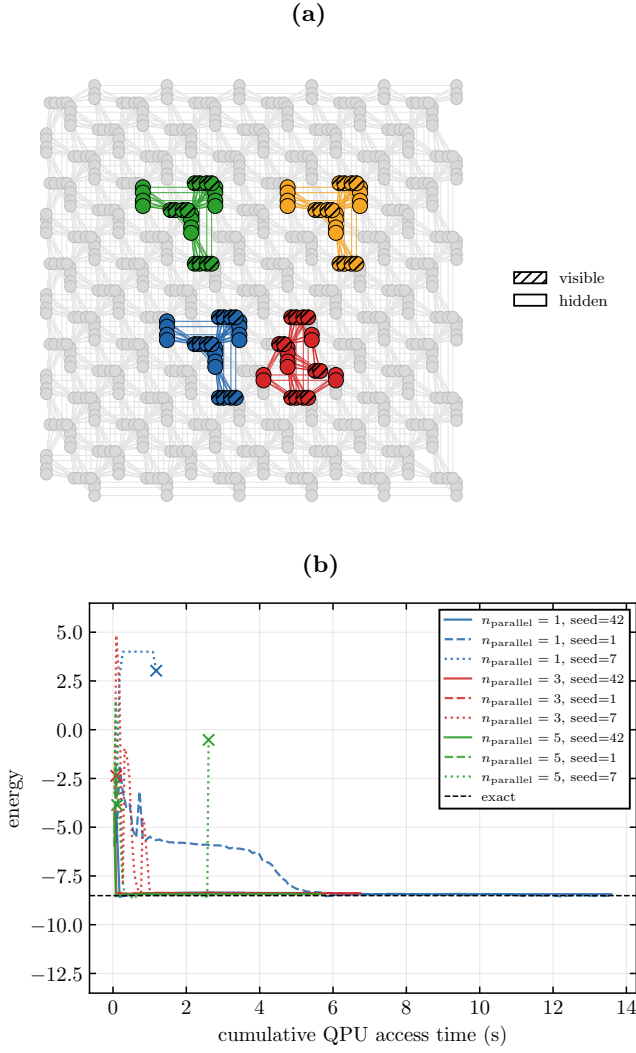
FIG. 8. (a) A four-copy Pegasus embedding layout. (b) All nine recorded training trajectories vs. cumulative QPU access time; crosses mark divergence.
