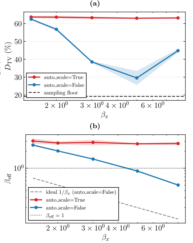
FIG. 1. Effect of automatic coefficient normalization on a small ( N = 8 ) Pegasus-embedded network. (a) Total-variation distance to the enumerated \pi_\theta . (b) Fitted \widehat{\beta}_{\text{LS}} (Eq. (6)). Disabling normalization lets the input scale \beta_x change the sampled law; enabling it cancels the attempted adjustment. The reference line is a finite-sample floor at this sample count, not a lower bound.
