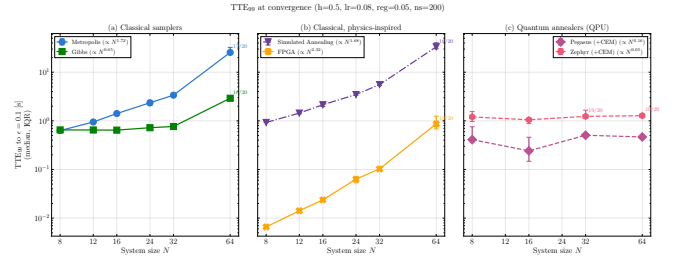
FIG. 6. TTE_{99} (Eq. (12)) vs. N at the single tested cell h = 0.5 , \epsilon = 0.1 . Annotated fractions give the successful-seed count where below 20/20. This is the only (\epsilon, h) cell for which a full- N curve currently exists; Sec. V B explains why it should not be read as representative.
