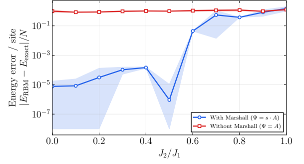
FIG. 9. Heisenberg energy error per spin, positive-amplitude vs. fixed-Marshall-sign ansatz, N = 8 , three seeds. Bands are recorded standard deviations.
