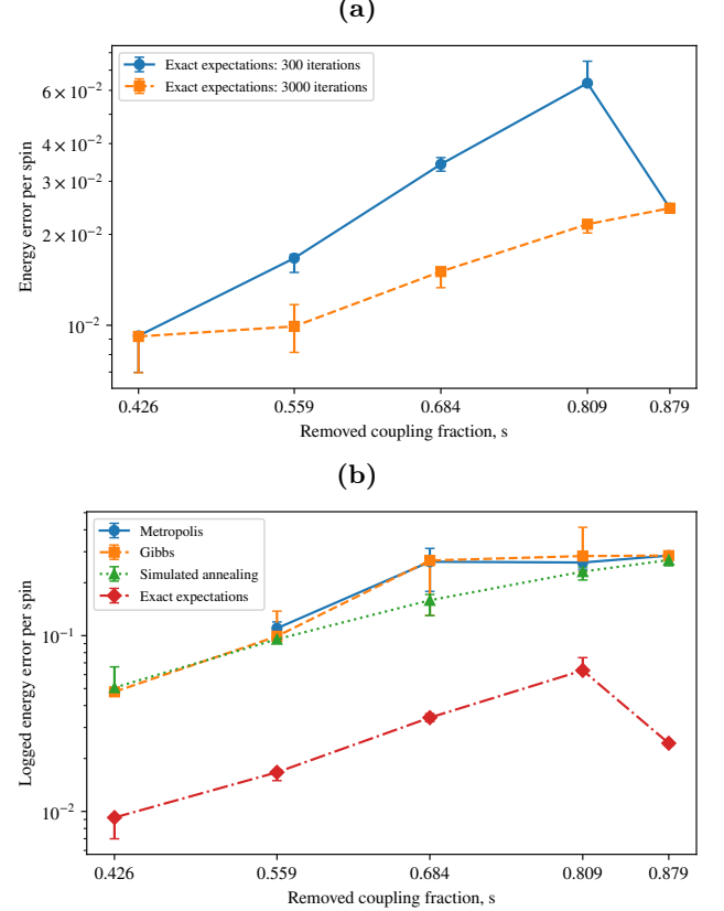
FIG. 7. (a) Exact-expectation training at 300 vs. 3000 iterations across sparsity masks. (b) Matched-iteration (300) comparison of exact expectations against three classical samplers. Five seeds per point; markers are medians, bars span first/third quartiles.
