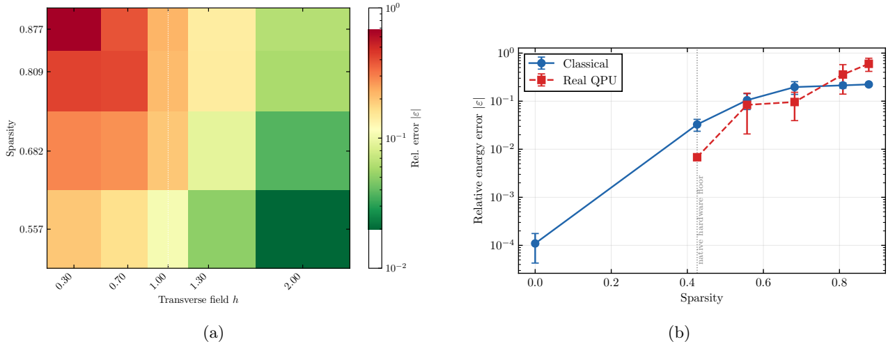
Figure 11: Error as a function of sparsity, with the number of hidden units kept equal t in both plots. (a) Error for different values of h . (b) Error at h = 1 , comparing classical training to training on the real QPU. The dotted line marks the lowest flows at this size.
