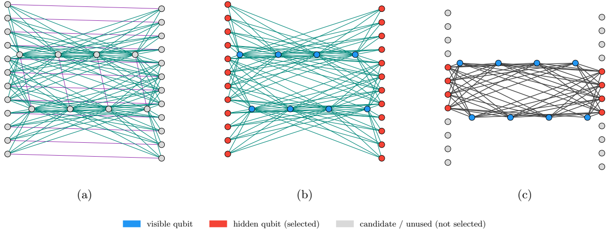
Figure 10: Construction of a chain-free sparse RBM from a D-Wave Zephyr hardware graph ( N = 8 visible units). (a) Identify internal couplers (green) and external/odd couplers (purple) (b) Creation of bipartite graph by restricting to internal couplers, splitting into hidden unit candidates (red) and visible units (blue). (c) RBM's visible-hidden connectivity mask by selecting the hidden units which maximize connectivity while keeping a min-set-cover. Non-selected candidates (grey) are dropped.
