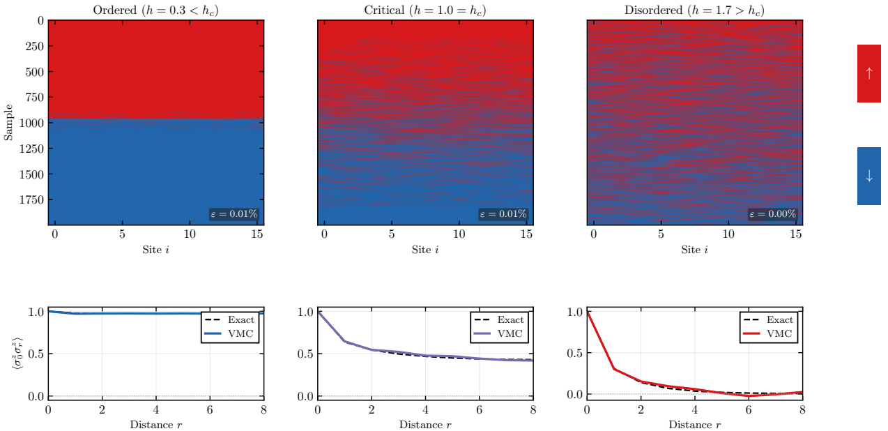
Figure 8: Spin configurations sampled from a trained RBM-VMC model for the one-dimensional Transverse-Field Ising Model (TFIM) at three values of the transverse field h . Top row: each column shows 2000 spin configurations \sigma \in \{-1, +1\}^N sampled from the learned wave function |\Psi_{\theta}|^2 , sorted by total magnetisation. Bottom row: spin-spin correlation C(r) = \langle \sigma_0^z \sigma_r^z \rangle as a function of distance r , computed from VMC samples (solid line) and exact diagonalisation (dashed line). The relative energy error \epsilon = |E_{\text{VMC}} - E_{\text{exact}}|/|E_{\text{exact}}| is shown in each panel. The model is a fully-connected RBM ( N = N_h = 16 ) trained for 300 iterations of Stochastic Reconfiguration with 500 Metropolis-Hastings samples per step.
