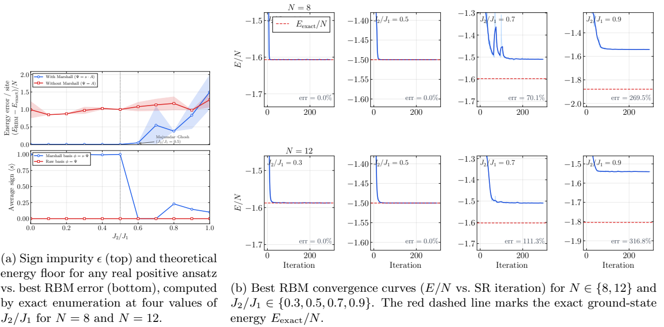
Figure 9: Visualization of the sign problem on the J_1 - J_2 Heisenberg chain. Left: sign impurity and overall training dynamics, Right: best run for selected instances.
