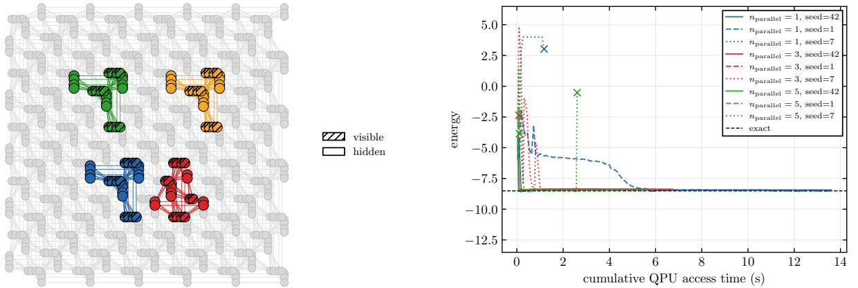
(b) Energy vs. cumulative QPU access time for n_{\text{parallel}} \in \{1, 3, 5\} , all 3 seeds shown individually. 'x' markers indicate a run diverged before reaching the plateau; among the seeds that converge, higher n_{\text{parallel}} reaches the plateau using less real QPU time.
