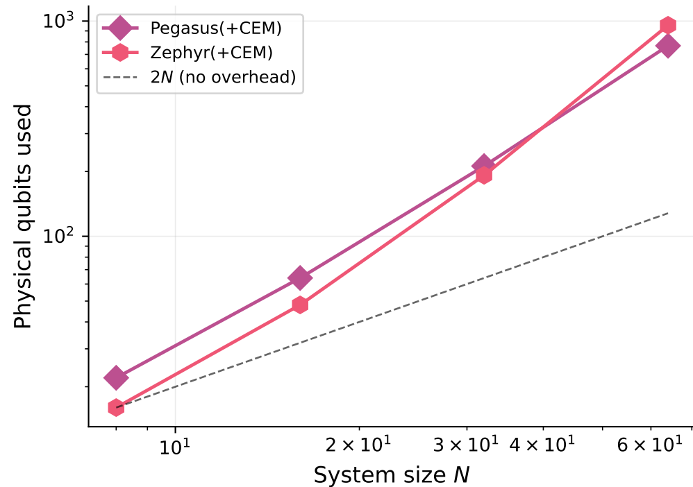
Physical qubits vs. N
