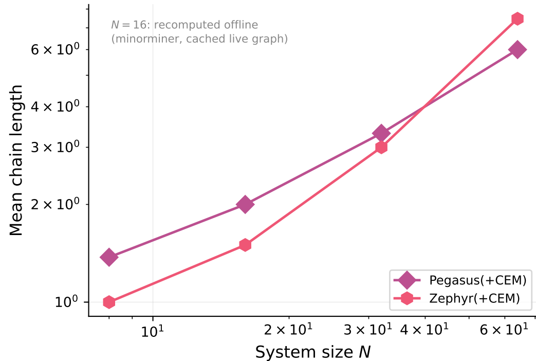
Mean chain length vs. N
